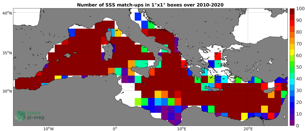
Figure 4: Number of SSS match-ups between Argo SSS and the SMOS SSS L3 v5 - 18 Days (CATDS-CECOS-LOCEAN) SSS product for the Mediterranean Sea Pi-MEP region over 1°x1° boxes and for the full satellite product period.
