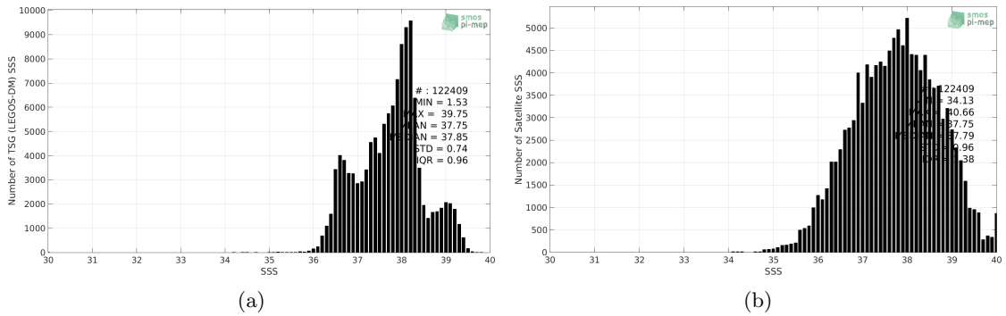
Figure 2: Histograms of SSS from TSG (LEGOS-DM) (a) and SMOS SSS L3 v4 - 9 Days (CATDS-CECOS-LOCEAN) (b) considering all match-up pairs per bins of 0.1 over the Mediterranean Sea Pi-MEP region and for the full satellite product period.
