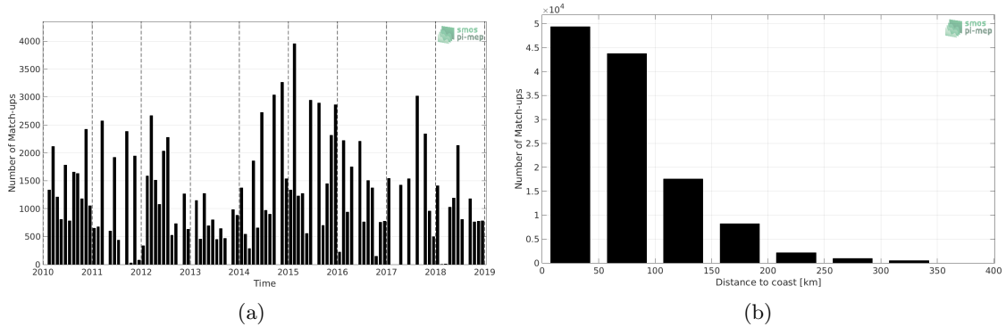
Figure 1: Number of match-ups between TSG (LEGOS-DM) and SMOS SSS L3 v4 - 9 Days (CATDS-CECOS-LOCEAN) SSS as a function of time (a) and as function of the distance to coast (b) over the Mediterranean Sea Pi-MEP region and for the full satellite product period.
