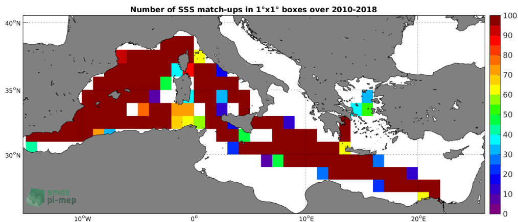
Figure 4: Number of SSS match-ups between TSG (LEGOS-DM) SSS and the SMOS SSS L3 v4 - 9 Days (CATDS-CECOS-LOCEAN) SSS product for the Mediterranean Sea Pi-MEP region over 1^\circ \times 1^\circ boxes and for the full satellite product period.
