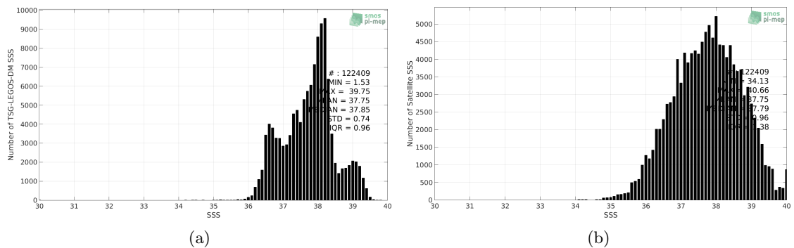
Figure 2: Histograms of SSS from TSG-LEGOS-DM (a) and SMOS-L3-CATDS-CECOS-LOCEAN-V4-9DAYS-25KM (b) considering all match-up pairs per bins of 0.1 over the Mediterranean Sea Pi-MEP region and for the full satellite product period.
