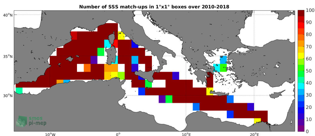
Figure 4: Number of SSS match-ups between TSG-LEGOS-DM SSS and the SMOS-L3-CATDS-CECOS-LOCEAN-V4-9DAYS-25KM SSS product for the Mediterranean Sea Pi-MEP region over 1^\circ \times 1^\circ boxes and for the full satellite product period.
