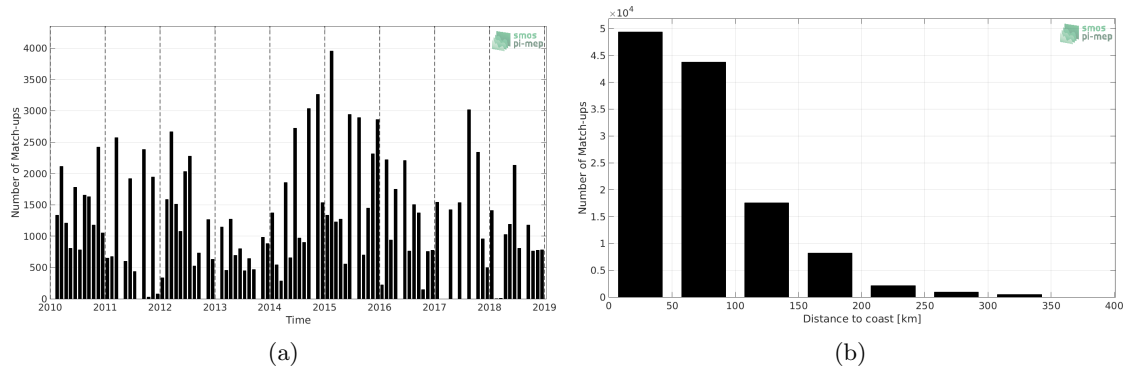
Figure 1: Number of match-ups between TSG-LEGOS-DM and SMOS-L3-CATDS-CECOS-LOCEAN-V4-9DAYS-25KM SSS as a function of time (a) and as function of the distance to coast (b) over the Mediterranean Sea Pi-MEP region and for the full satellite product period.
