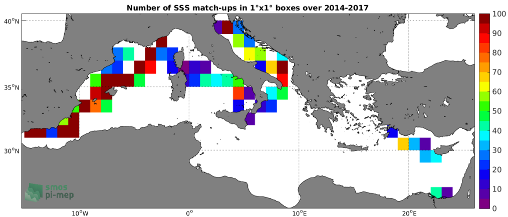
Figure 4: Number of SSS match-ups between TSG (GOSUD-Sailing-ship) SSS and the SMOS SSS L3 v4 - 9 Days (CATDS-CECOS-LOCEAN) SSS product for the Mediterranean Sea Pi-MEP region over 1^\circ \times 1^\circ boxes and for the full satellite product period.
