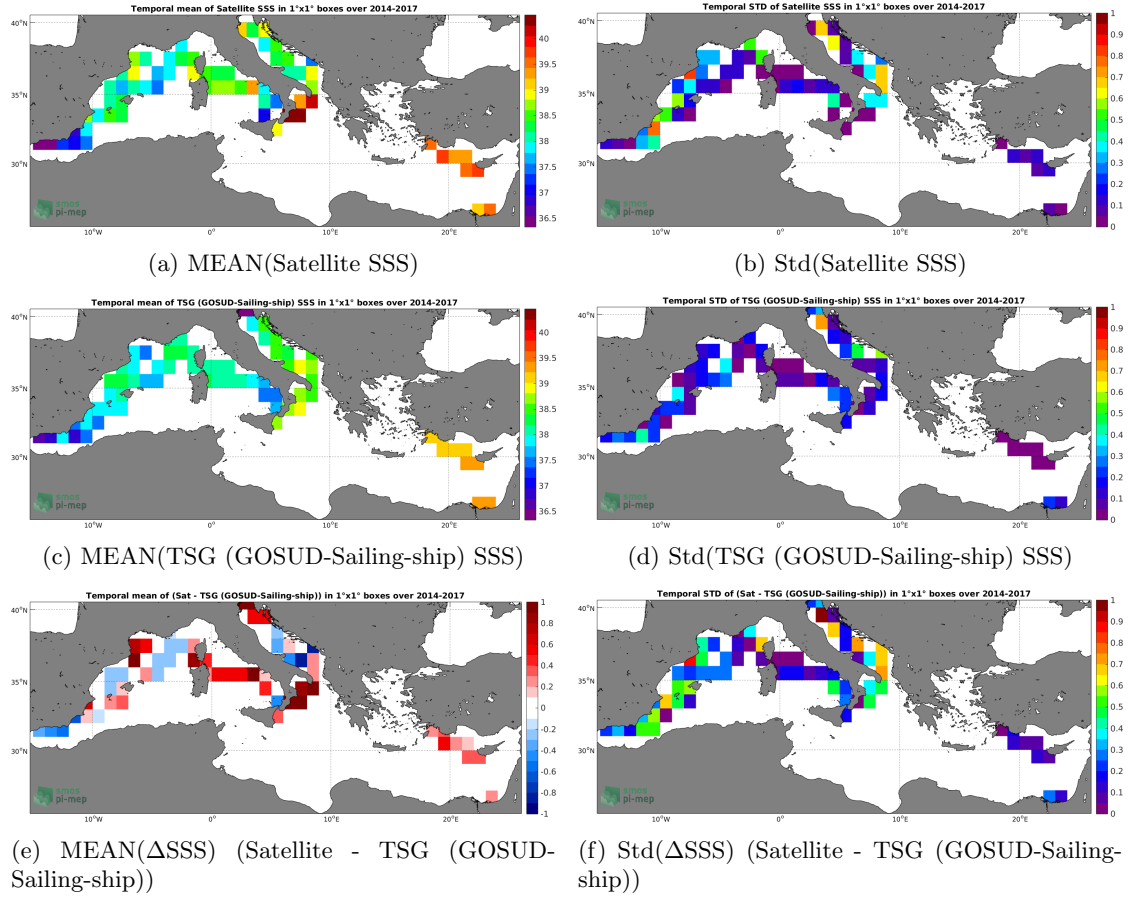
Figure 6: Temporal mean (left) and Std (right) of SSS from SMOS SSS L3 v4 - 9 Days (CATDS-CECOS-LOCEAN) (top), TSG (GOSUD-Sailing-ship) (middle), and of \Delta SSS (Satellite - TSG (GOSUD-Sailing-ship)). Only match-up pairs are used to generate these maps.
