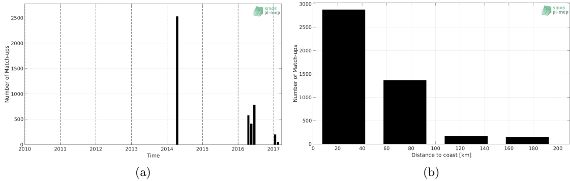
Figure 1: Number of match-ups between TSG (GOSUD-Sailing-ship) and SMOS SSS L3 v4 - 9 Days (CATDS-CECOS-LOCEAN) SSS as a function of time (a) and as function of the distance to coast (b) over the Mediterranean Sea Pi-MEP region and for the full satellite product period.
