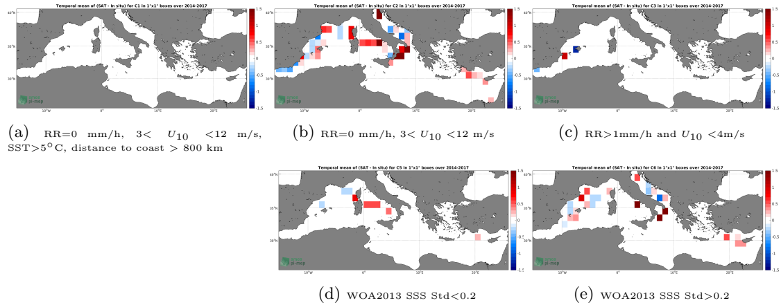
Figure 12: Temporal mean gridded over spatial boxes of size 1^\circ \times 1^\circ of \Delta SSS (SMOS SSS L3 v4 - 9 Days (CATDS-CECOS-LOCEAN) - TSG (GOSUD-Sailing-ship)) for 5 different subdatasets corresponding to:RR=0 mm/h, 3 < U_{10} < 12 m/s, SST >5^\circ\text{C} , distance to coast > 800 km (a), RR=0 mm/h, 3 < U_{10} < 12 m/s (b), RR >1 mm/h and U_{10} < 4 m/s (c), WOA2013 SSS Std <0.2 (d), WOA2013 SSS Std >0.2 (e).
