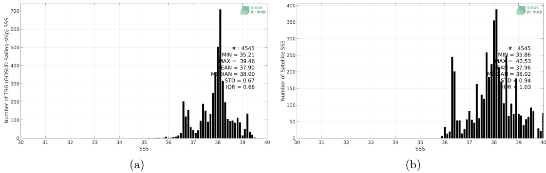
Figure 2: Histograms of SSS from TSG (GOSUD-Sailing-ship) (a) and SMOS SSS L3 v4 - 9 Days (CATDS-CECOS-LOCEAN) (b) considering all match-up pairs per bins of 0.1 over the Mediterranean Sea Pi-MEP region and for the full satellite product period.
