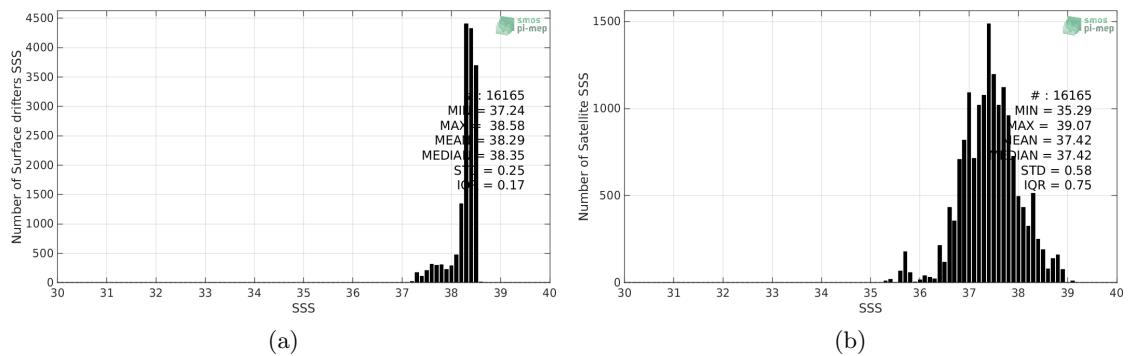
Figure 2: Histograms of SSS from Surface drifters (a) and SMOS-L3-CATDS-CECOS-LOCEAN-V4-9DAYS-25KM (b) considering all match-up pairs per bins of 0.1 over the Mediterranean Sea Pi-MEP region and for the full satellite product period.
