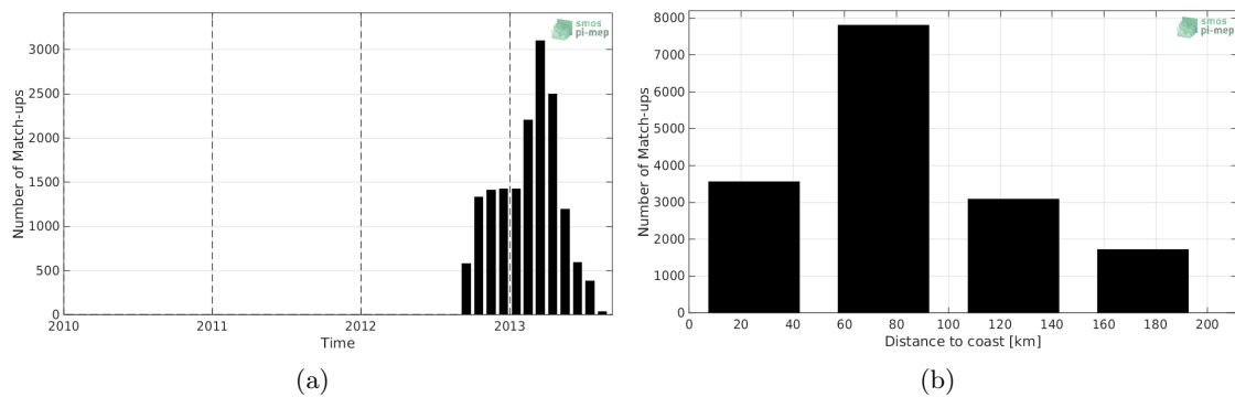
Figure 1: Number of match-ups between Surface drifters and SMOS-L3-CATDS-CECOS-LOCEAN-V4-9DAYS-25KM SSS as a function of time (a) and as function of the distance to coast (b) over the Mediterranean Sea Pi-MEP region and for the full satellite product period.
