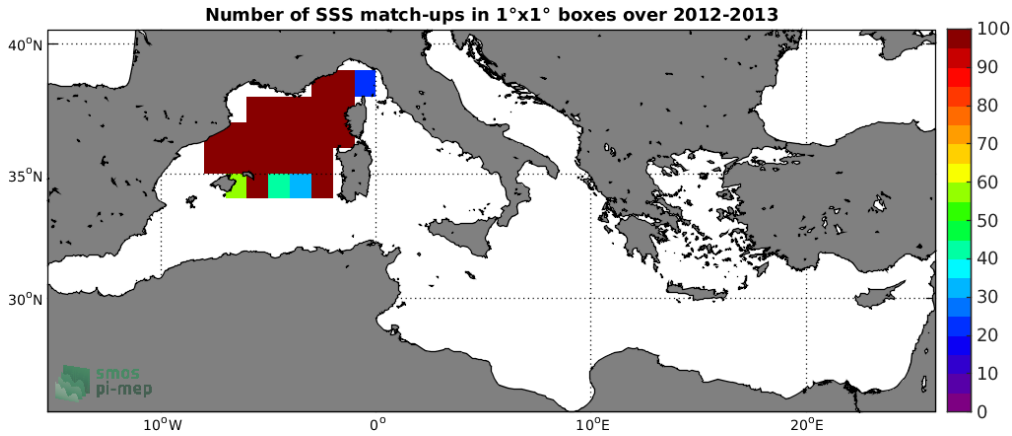
Figure 3: Number of SSS match-ups between Surface drifters SSS and the SMOS-L3-CATDS-CECOS-LOCEAN-V4-9DAYS-25KM SSS product for the Mediterranean Sea Pi-MEP region over 1^\circ \times 1^\circ boxes and for the full satellite product period.
