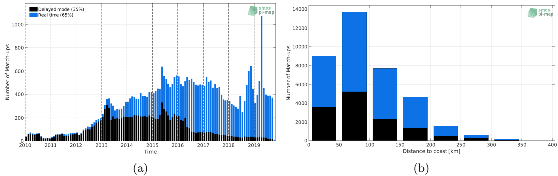
Figure 1: Number of match-ups between Argo and SMOS-L3-CATDS-CECOS-LOCEAN-V4-9DAYS-25KM SSS as a function of time (a) and as function of the distance to coast (b) over the Mediterranean Sea Pi-MEP region and for the full satellite product period.
