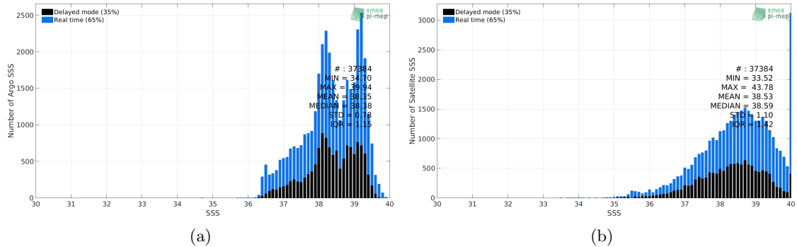
Figure 2: Histograms of SSS from Argo (a) and SMOS-L3-CATDS-CECOS-LOCEAN-V4-9DAYS-25KM (b) considering all match-up pairs per bins of 0.1 over the Mediterranean Sea Pi-MEP region and for the full satellite product period.
