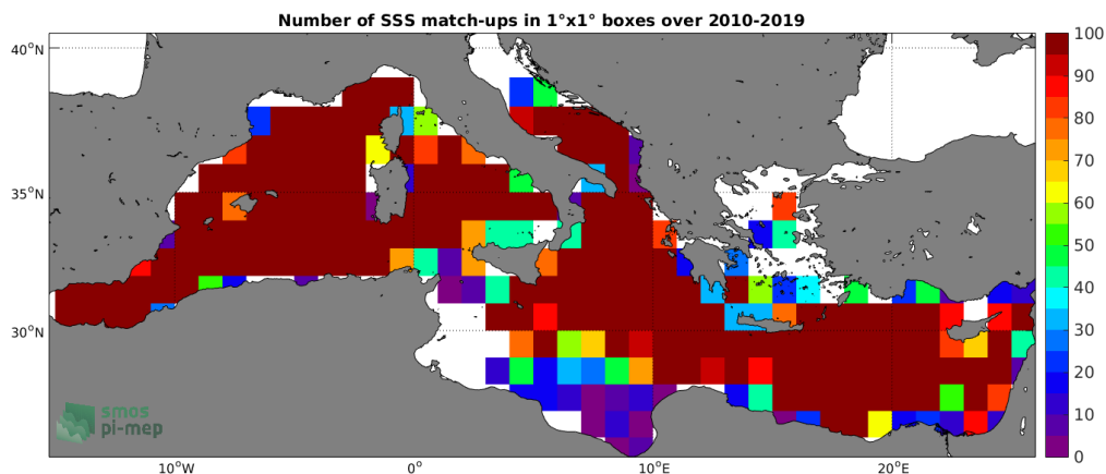
Figure 4: Number of SSS match-ups between Argo SSS and the SMOS-L3-CATDS-CECOS-LOCEAN-V4-9DAYS-25KM SSS product for the Mediterranean Sea Pi-MEP region over 1°x1° boxes and for the full satellite product period.
