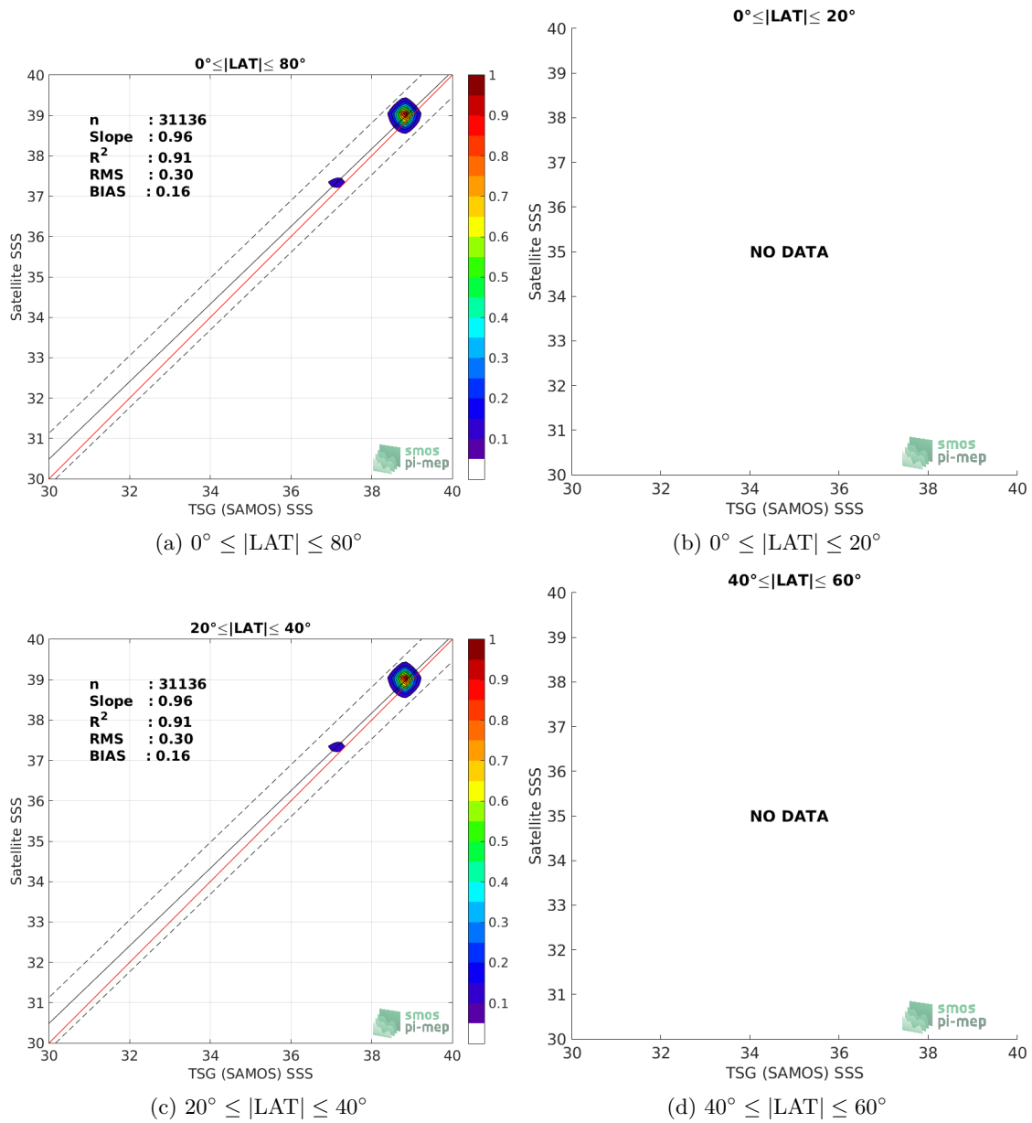
Figure 9: Contour maps of the concentration of SMOS SSS L3 v4 - 18 Days (CATDS-CECOS-LOCEAN) SSS (y-axis) versus TSG (SAMOS) SSS (x-axis) at match-up pairs for different latitude bands. For each plot, the red line shows x=y . The black thin and dashed lines indicate a linear fit through the data cloud and the \pm 95\% confidence levels, respectively. The number match-up pairs n , the slope and R^2 coefficient of the linear fit, the root mean square (RMS) and the mean bias between satellite and in situ data are indicated for each latitude band in each plots.
