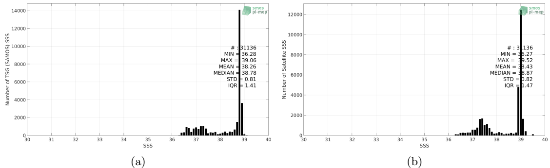
Figure 2: Histograms of SSS from TSG (SAMOS) (a) and SMOS SSS L3 v4 - 18 Days (CATDS-CECOS-LOCEAN) (b) considering all match-up pairs per bins of 0.1 over the Mediterranean Sea Pi-MEP region and for the full satellite product period.
