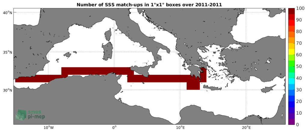
Figure 4: Number of SSS match-ups between TSG (SAMOS) SSS and the SMOS SSS L3 v4 - 18 Days (CATDS-CECOS-LOCEAN) SSS product for the Mediterranean Sea Pi-MEP region over 1^\circ \times 1^\circ boxes and for the full satellite product period.
