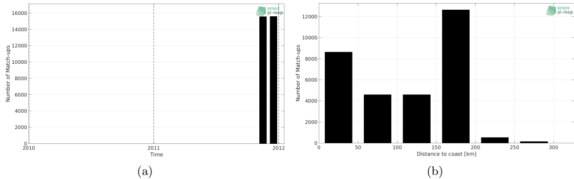
Figure 1: Number of match-ups between TSG (SAMOS) and SMOS SSS L3 v4 - 18 Days (CATDS-CECOS-LOCEAN) SSS as a function of time (a) and as function of the distance to coast (b) over the Mediterranean Sea Pi-MEP region and for the full satellite product period.
