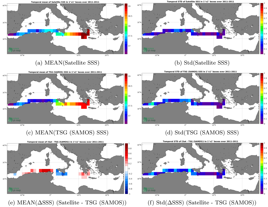
Figure 6: Temporal mean (left) and Std (right) of SSS from SMOS SSS L3 v4 - 18 Days (CATDS-CECOS-LOCEAN) (top), TSG (SAMOS) (middle), and of \Delta SSS (Satellite - TSG (SAMOS)). Only match-up pairs are used to generate these maps.
