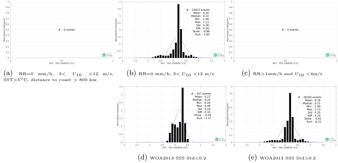
Figure 13: Normalized histogram of \Delta SSS (SMOS SSS L3 v4 - 18 Days (CATDS-CECOS-LOCEAN) - TSG (SAMOS)) for 5 different subdatasets corresponding to: RR=0 mm/h, 3 < U_{10} < 12 m/s, SST > 5°C, distance to coast > 800 km (a), RR=0 mm/h, 3 < U_{10} < 12 m/s (b), RR > 1mm/h and U_{10} < 4 m/s (c), WOA2013 SSS Std < 0.2 (d), WOA2013 SSS Std > 0.2 (e).
