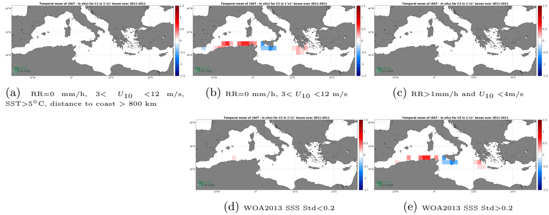
Figure 12: Temporal mean gridded over spatial boxes of size 1^{\circ}\times 1^{\circ} of \Delta\text{SSS} (SMOS SSS L3 v4 - 18 Days (CATDS-CECOS-LOCEAN) - TSG (SAMOS)) for 5 different subdatasets corresponding to:RR=0 mm/h, 3 < U_{10} < 12 m/s, SST >5^{\circ}\text{C} , distance to coast > 800 km (a), RR=0 mm/h, 3 < U_{10} < 12 m/s (b), RR >1 mm/h and U_{10} < 4 m/s (c), WOA2013 SSS Std <0.2 (d), WOA2013 SSS Std >0.2 (e).
