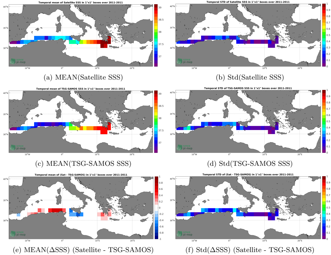
Figure 6: Temporal mean (left) and Std (right) of SSS from SMOS-L3-CATDS-CECOS-LOCEAN-V4-18DAYS-25KM (top), TSG-SAMOS (middle), and of \Delta SSS (Satellite - TSG-SAMOS). Only match-up pairs are used to generate these maps.
