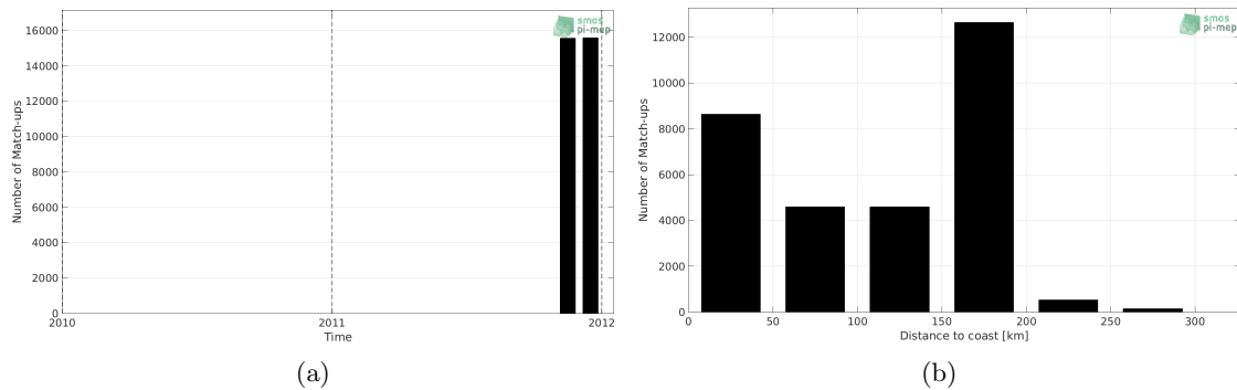
Figure 1: Number of match-ups between TSG-SAMOS and SMOS-L3-CATDS-CECOS-LOCEAN-V4-18DAYS-25KM SSS as a function of time (a) and as function of the distance to coast (b) over the Mediterranean Sea Pi-MEP region and for the full satellite product period.
