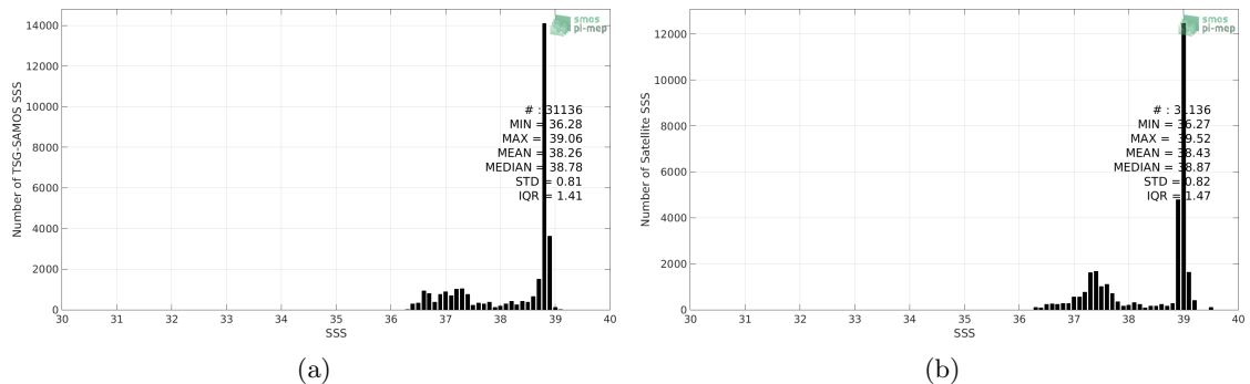
Figure 2: Histograms of SSS from TSG-SAMOS (a) and SMOS-L3-CATDS-CECOS-LOCEAN-V4-18DAYS-25KM (b) considering all match-up pairs per bins of 0.1 over the Mediterranean Sea Pi-MEP region and for the full satellite product period.
