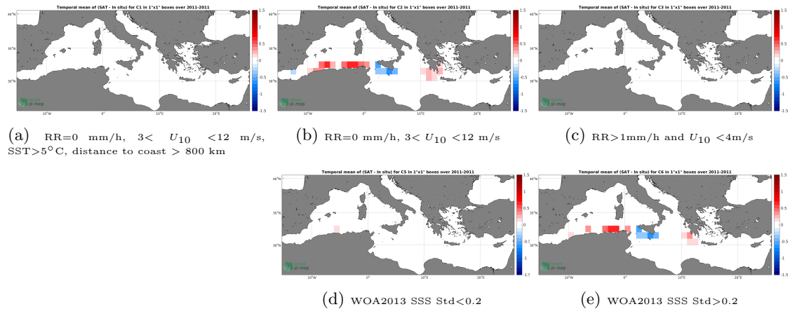
Figure 12: Temporal mean gridded over spatial boxes of size 1^{\circ}\times 1^{\circ} of \Delta\text{SSS} (SMOS-L3-CATDS-CECOS-LOCEAN-V4-18DAYS-25KM - TSG-SAMOS) for 5 different subdatasets corresponding to:RR=0 mm/h, 3 < U_{10} < 12 m/s, SST > 5^{\circ}\text{C} , distance to coast > 800 km (a), RR=0 mm/h, 3 < U_{10} < 12 m/s (b), RR > 1 mm/h and U_{10} < 4 m/s (c), WOA2013 SSS Std < 0.2 (d), WOA2013 SSS Std > 0.2 (e).
