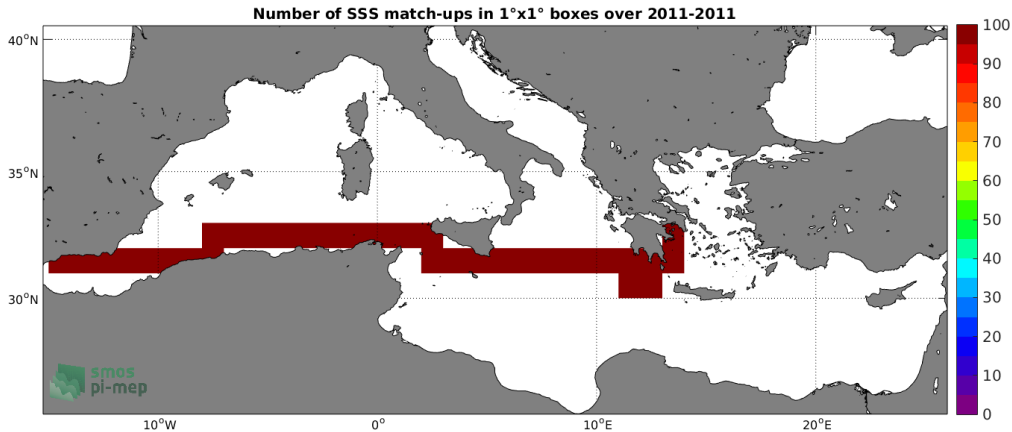
Figure 4: Number of SSS match-ups between TSG-SAMOS SSS and the SMOS-L3-CATDS-CECOS-LOCEAN-V4-18DAYS-25KM SSS product for the Mediterranean Sea Pi-MEP region over 1°x1° boxes and for the full satellite product period.
