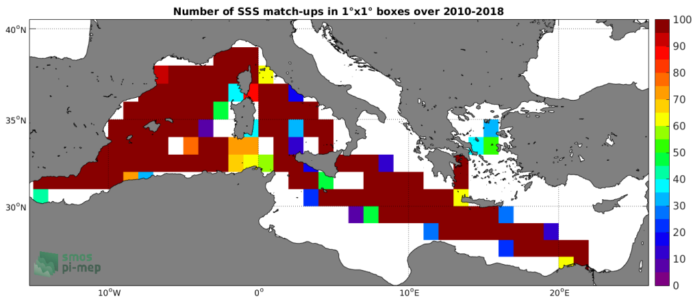
Figure 4: Number of SSS match-ups between TSG-LEGOS-DM SSS and the SMOS-L3-CATDS-CECOS-LOCEAN-V4-18DAYS-25KM SSS product for the Mediterranean Sea Pi-MEP region over 1^\circ \times 1^\circ boxes and for the full satellite product period.
