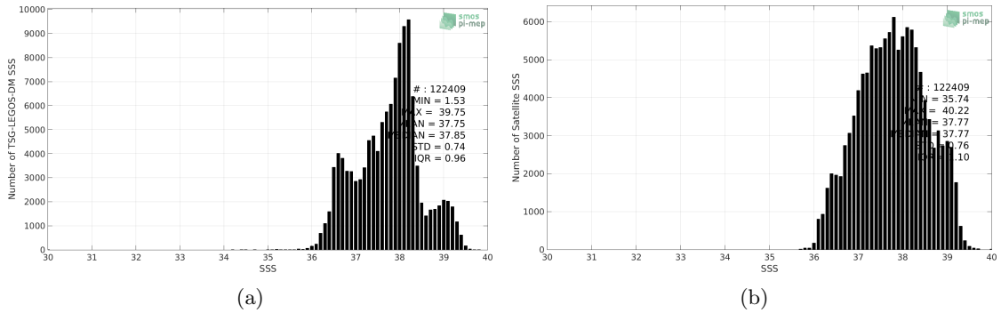
Figure 2: Histograms of SSS from TSG-LEGOS-DM (a) and SMOS-L3-CATDS-CECOS-LOCEAN-V4-18DAYS-25KM (b) considering all match-up pairs per bins of 0.1 over the Mediterranean Sea Pi-MEP region and for the full satellite product period.
