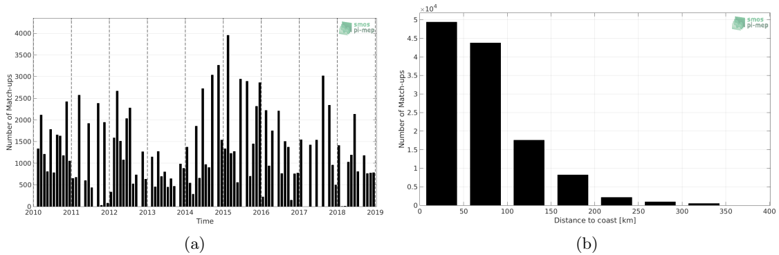
Figure 1: Number of match-ups between TSG-LEGOS-DM and SMOS-L3-CATDS-CECOS-LOCEAN-V4-18DAYS-25KM SSS as a function of time (a) and as function of the distance to coast (b) over the Mediterranean Sea Pi-MEP region and for the full satellite product period.
