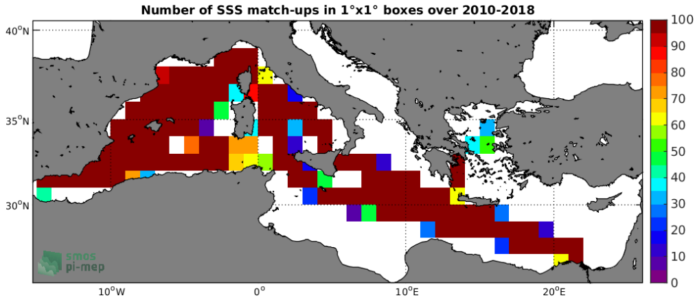
Figure 4: Number of SSS match-ups between TSG-LEGOS-DM SSS and the SMOS-L3-CATDS-CECOS-LOCEAN-V4-18DAYS-25KM SSS product for the Mediterranean Sea Pi-MEP region over 1°x1° boxes and for the full satellite product period.
