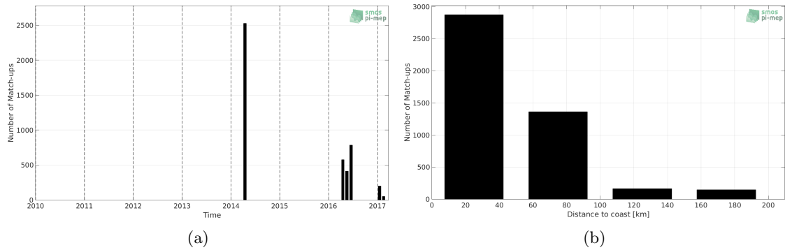
Figure 1: Number of match-ups between TSG (GOSUD-Sailing-ship) and SMOS SSS L3 v4 - 18 Days (CATDS-CECOS-LOCEAN) SSS as a function of time (a) and as function of the distance to coast (b) over the Mediterranean Sea Pi-MEP region and for the full satellite product period.
