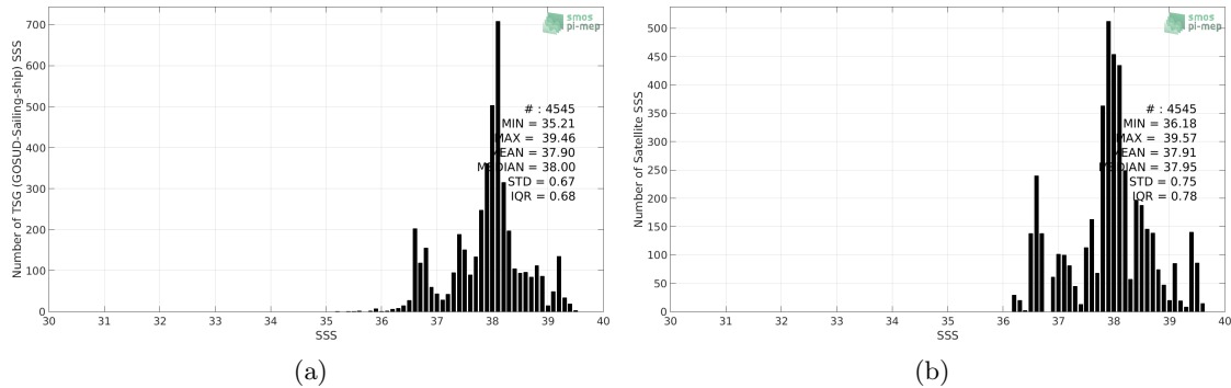
Figure 2: Histograms of SSS from TSG (GOSUD-Sailing-ship) (a) and SMOS SSS L3 v4 - 18 Days (CATDS-CECOS-LOCEAN) (b) considering all match-up pairs per bins of 0.1 over the Mediterranean Sea Pi-MEP region and for the full satellite product period.
