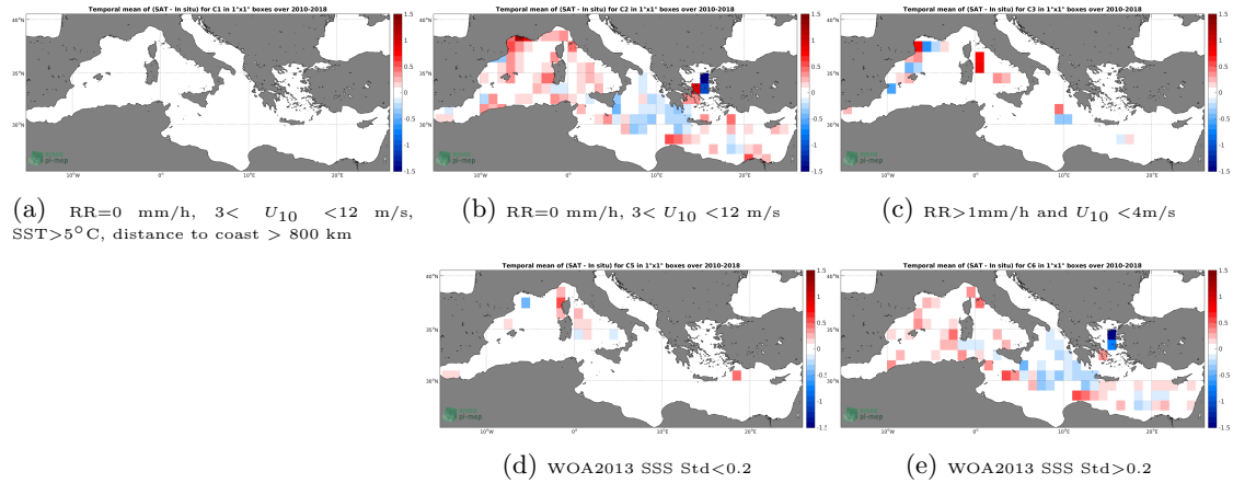
Figure 12: Temporal mean gridded over spatial boxes of size 1^\circ \times 1^\circ of \Delta SSS (SMOS SSS L3 v4 - 18 Days (CATDS-CECOS-LOCEAN) - TSG (GOSUD-Research-vessel)) for 5 different subdatasets corresponding to:RR=0 mm/h, 3 < U_{10} < 12 m/s, SST >5^\circ\text{C} , distance to coast > 800 km (a), RR=0 mm/h, 3 < U_{10} < 12 m/s (b), RR >1 mm/h and U_{10} < 4 m/s (c), WOA2013 SSS Std <0.2 (d), WOA2013 SSS Std >0.2 (e).
