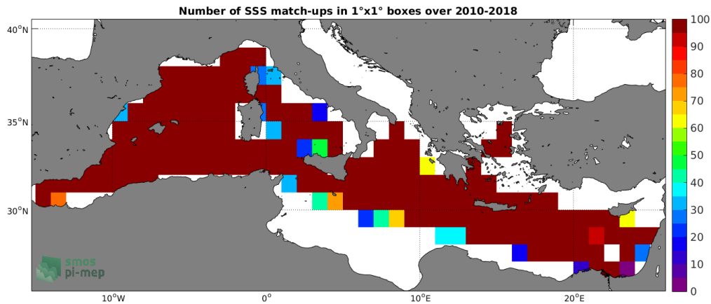
Figure 4: Number of SSS match-ups between TSG (GOSUD-Research-vessel) SSS and the SMOS SSS L3 v4 - 18 Days (CATDS-CECOS-LOCEAN) SSS product for the Mediterranean Sea Pi-MEP region over 1^\circ \times 1^\circ boxes and for the full satellite product period.
