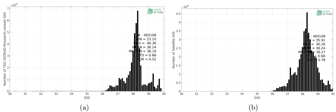
Figure 2: Histograms of SSS from TSG (GOSUD-Research-vessel) (a) and SMOS SSS L3 v4 - 18 Days (CATDS-CECOS-LOCEAN) (b) considering all match-up pairs per bins of 0.1 over the Mediterranean Sea Pi-MEP region and for the full satellite product period.
