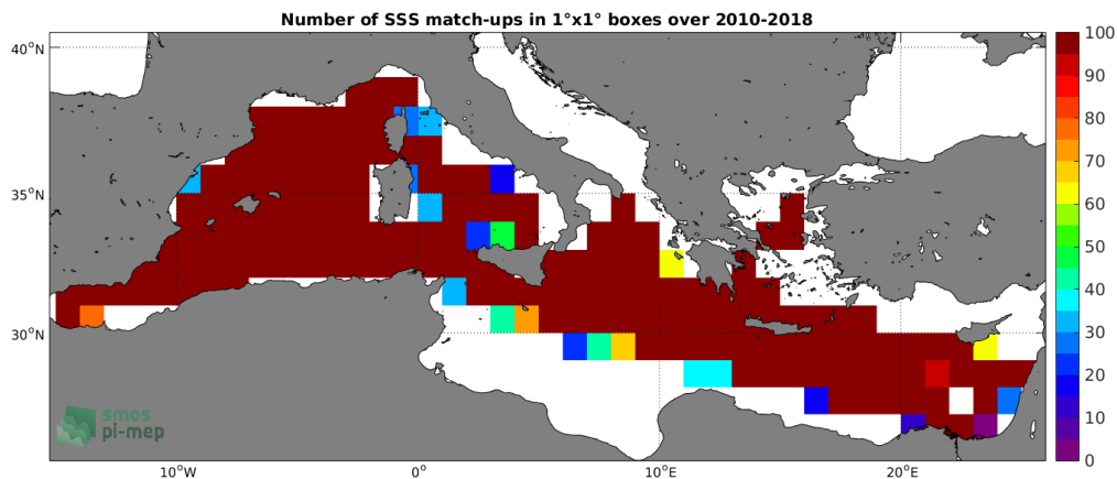
Figure 4: Number of SSS match-ups between TSG-GOSUD-Research-vessel SSS and the SMOS-L3-CATDS-CECOS-LOCEAN-V4-18DAYS-25KM SSS product for the Mediterranean Sea Pi-MEP region over 1^\circ \times 1^\circ boxes and for the full satellite product period.
