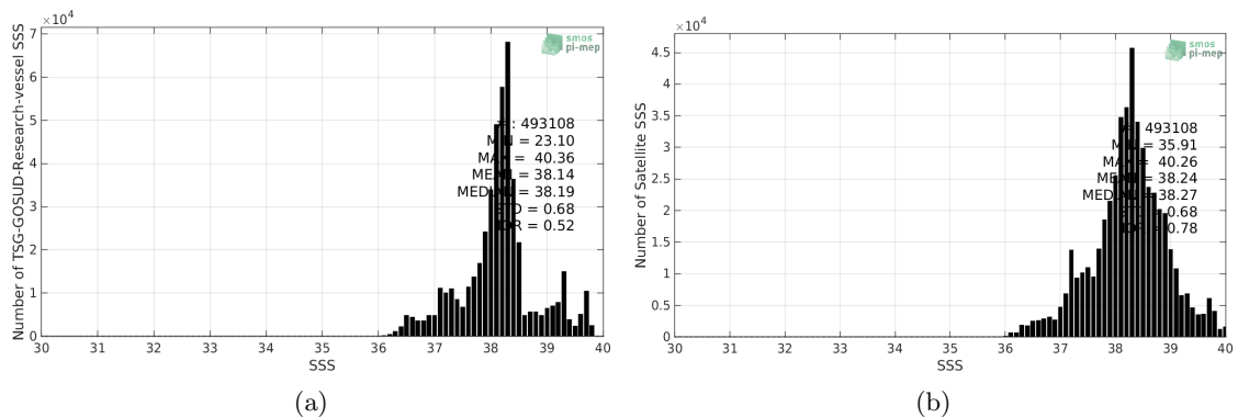
Figure 2: Histograms of SSS from TSG-GOSUD-Research-vessel (a) and SMOS-L3-CATDS-CECOS-LOCEAN-V4-18DAYS-25KM (b) considering all match-up pairs per bins of 0.1 over the Mediterranean Sea Pi-MEP region and for the full satellite product period.
