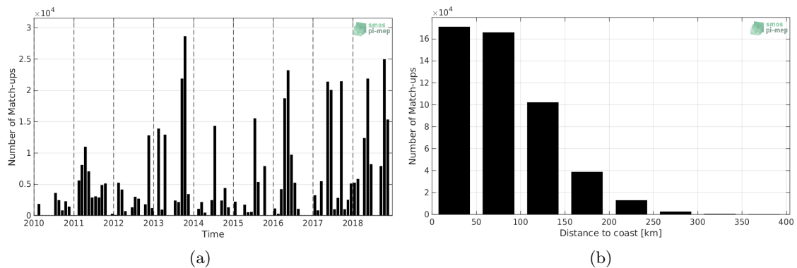
Figure 1: Number of match-ups between TSG-GOSUD-Research-vessel and SMOS-L3-CATDS-CECOS-LOCEAN-V4-18DAYS-25KM SSS as a function of time (a) and as function of the distance to coast (b) over the Mediterranean Sea Pi-MEP region and for the full satellite product period.
