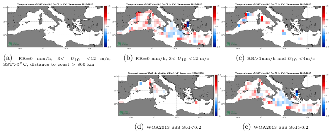
Figure 12: Temporal mean gridded over spatial boxes of size 1^\circ \times 1^\circ of \Delta SSS (SMOS-L3-CATDS-CECOS-LOCEAN-V4-18DAYS-25KM - TSG-GOSUD-Research-vessel) for 5 different subdatasets corresponding to:RR=0 mm/h, 3 < U_{10} < 12 m/s, SST >5^\circ\text{C} , distance to coast > 800 km (a), RR=0 mm/h, 3 < U_{10} < 12 m/s (b), RR >1 mm/h and U_{10} < 4 m/s (c), WOA2013 SSS Std <0.2 (d), WOA2013 SSS Std >0.2 (e).
