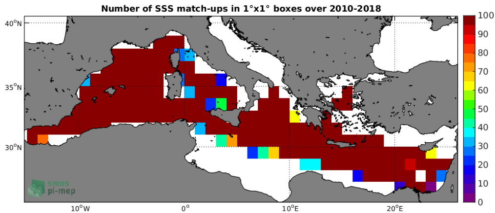
Figure 4: Number of SSS match-ups between TSG-GOSUD-Research-vessel SSS and the SMOS-L3-CATDS-CECOS-LOCEAN-V4-18DAYS-25KM SSS product for the Mediterranean Sea Pi-MEP region over 1°x1° boxes and for the full satellite product period.
