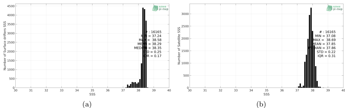
Figure 2: Histograms of SSS from Surface drifters (a) and SMOS-L3-CATDS-CECOS-LOCEAN-V4-18DAYS-25KM (b) considering all match-up pairs per bins of 0.1 over the Mediterranean Sea Pi-MEP region and for the full satellite product period.
