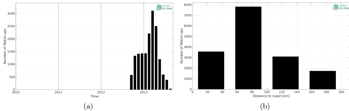
Figure 1: Number of match-ups between Surface drifters and SMOS-L3-CATDS-CECOS-LOCEAN-V4-18DAYS-25KM SSS as a function of time (a) and as function of the distance to coast (b) over the Mediterranean Sea Pi-MEP region and for the full satellite product period.
