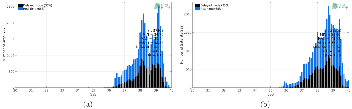
Figure 2: Histograms of SSS from Argo (a) and SMOS SSS L3 v4 - 18 Days (CATDS-CECOS-LOCEAN) (b) considering all match-up pairs per bins of 0.1 over the Mediterranean Sea Pi-MEP region and for the full satellite product period.
