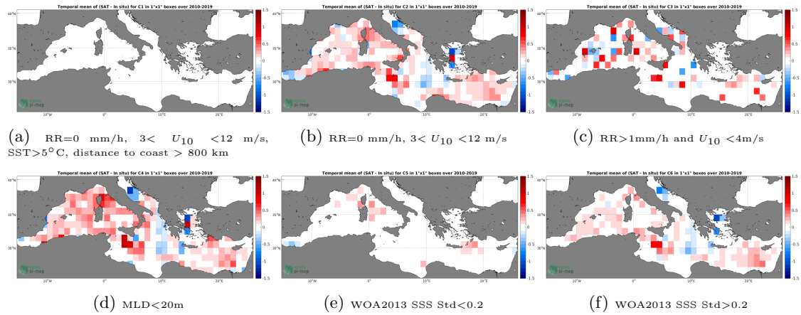
Figure 12: Temporal mean gridded over spatial boxes of size 1^\circ \times 1^\circ of \Delta SSS (SMOS SSS L3 v4 - 18 Days (CATDS-CECOS-LOCEAN) - Argo) for 6 different subdatasets corresponding to:RR=0 mm/h, 3 < U_{10} < 12 m/s, SST >5^\circ\text{C} , distance to coast > 800 km (a), RR=0 mm/h, 3 < U_{10} < 12 m/s (b), RR >1 mm/h and U_{10} < 4 m/s (c),MLD <20 m (d),WOA2013 SSS Std <0.2 (e),WOA2013 SSS Std >0.2 (f).
