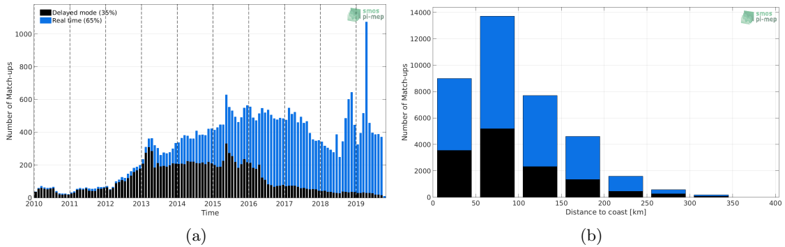
Figure 1: Number of match-ups between Argo and SMOS SSS L3 v4 - 18 Days (CATDS-CECOS-LOCEAN) SSS as a function of time (a) and as function of the distance to coast (b) over the Mediterranean Sea Pi-MEP region and for the full satellite product period.
