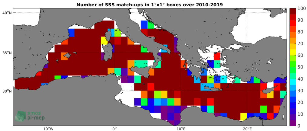
Figure 4: Number of SSS match-ups between Argo SSS and the SMOS SSS L3 v4 - 18 Days (CATDS-CECOS-LOCEAN) SSS product for the Mediterranean Sea Pi-MEP region over 1°x1° boxes and for the full satellite product period.
