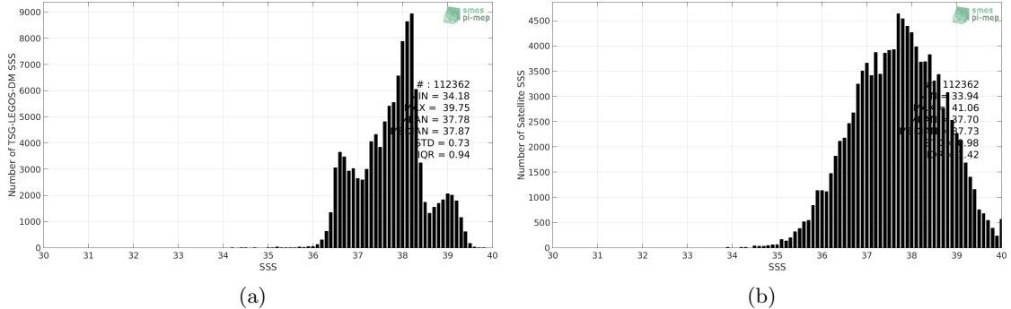
Figure 2: Histograms of SSS from TSG-LEGOS-DM (a) and SMOS-L3-CATDS-CECOS-LOCEAN-V3-9DAYS-25KM (b) considering all match-up pairs per bins of 0.1 over the Mediterranean Sea Pi-MEP region and for the full satellite product period.
