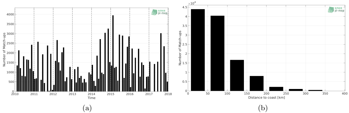
Figure 1: Number of match-ups between TSG-LEGOS-DM and SMOS-L3-CATDS-CECOS-LOCEAN-V3-9DAYS-25KM SSS as a function of time (a) and as function of the distance to coast (b) over the Mediterranean Sea Pi-MEP region and for the full satellite product period.
