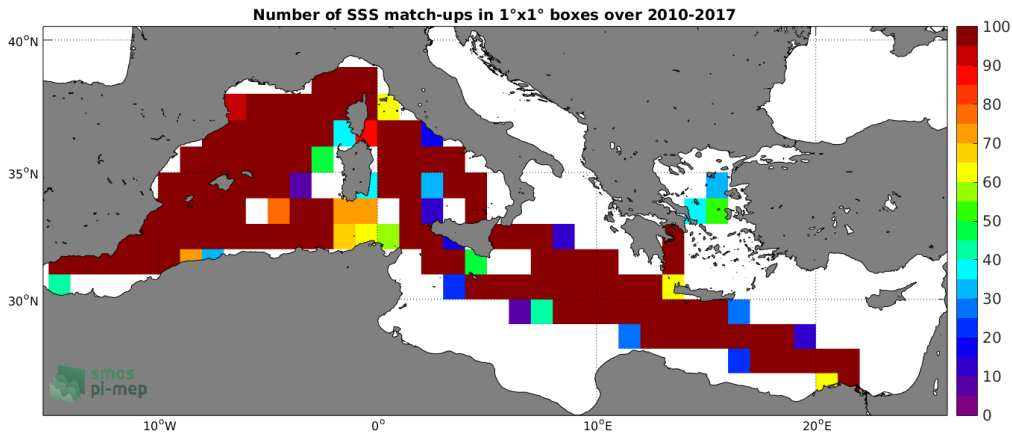
Figure 4: Number of SSS match-ups between TSG-LEGOS-DM SSS and the SMOS-L3-CATDS-CECOS-LOCEAN-V3-9DAYS-25KM SSS product for the Mediterranean Sea Pi-MEP region over 1^\circ \times 1^\circ boxes and for the full satellite product period.
