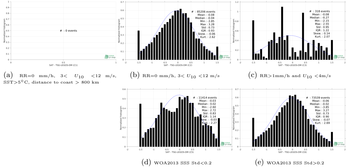
Figure 13: Normalized histogram of \Delta SSS (SMOS-L3-CATDS-CECOS-LOCEAN-V3-9DAYS-25KM - TSG-LEGOS-DM) for 5 different subdatasets corresponding to: RR=0 mm/h, 3 < U_{10} < 12 m/s, SST > 5°C, distance to coast > 800 km (a), RR=0 mm/h, 3 < U_{10} < 12 m/s (b), RR > 1mm/h and U_{10} < 4 m/s (c), WOA2013 SSS Std < 0.2 (d), WOA2013 SSS Std > 0.2 (e).
