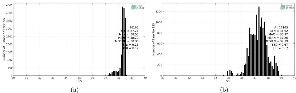
Figure 2: Histograms of SSS from Surface drifters (a) and SMOS-L3-CATDS-CECOS-LOCEAN-V3-9DAYS-25KM (b) considering all match-up pairs per bins of 0.1 over the Mediterranean Sea Pi-MEP region and for the full satellite product period.
