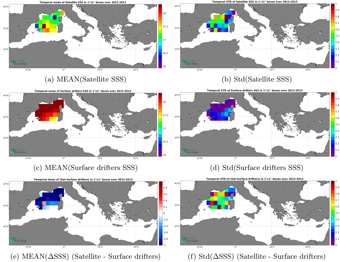
Figure 5: Temporal mean (left) and Std (right) of SSS from SMOS-L3-CATDS-CECOS-LOCEAN-V3-9DAYS-25KM (top), Surface drifters (middle), and of \Delta SSS (Satellite - Surface drifters). Only match-up pairs are used to generate these maps.
