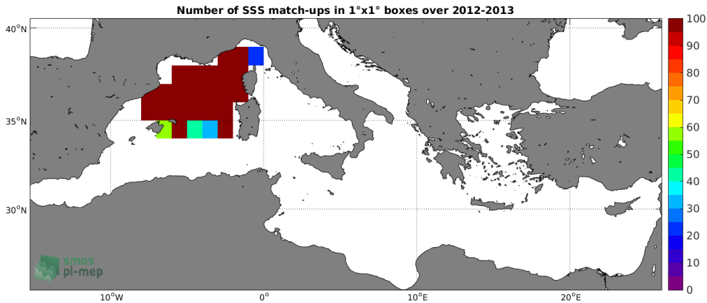
Figure 3: Number of SSS match-ups between Surface drifters SSS and the SMOS-L3-CATDS-CECOS-LOCEAN-V3-9DAYS-25KM SSS product for the Mediterranean Sea Pi-MEP region over 1^\circ \times 1^\circ boxes and for the full satellite product period.
