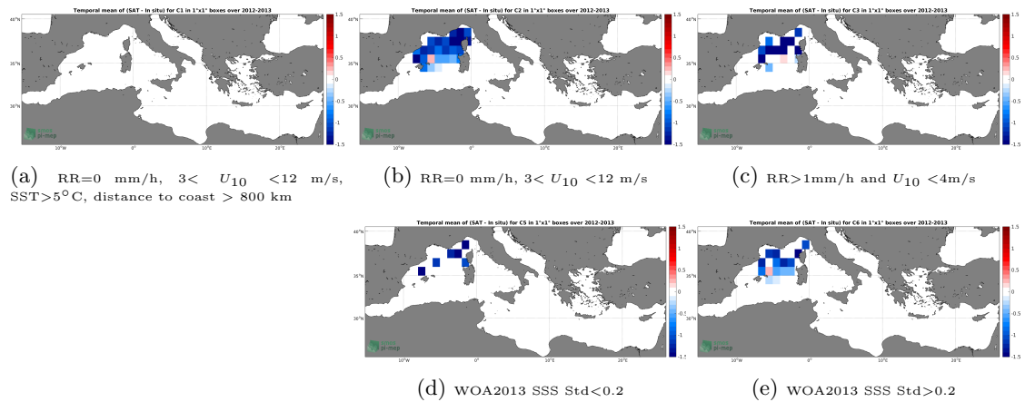
Figure 11: Temporal mean gridded over spatial boxes of size 1^\circ \times 1^\circ of \Delta SSS (SMOS-L3-CATDS-CECOS-LOCEAN-V3-9DAYS-25KM - Surface drifters) for 5 different subdatasets corresponding to:RR=0 mm/h, 3 < U_{10} < 12 m/s, SST >5^\circ C, distance to coast > 800 km (a), RR=0 mm/h, 3 < U_{10} < 12 m/s (b), RR >1 mm/h and U_{10} < 4 m/s (c), WOA2013 SSS Std <0.2 (d), WOA2013 SSS Std >0.2 (e).
