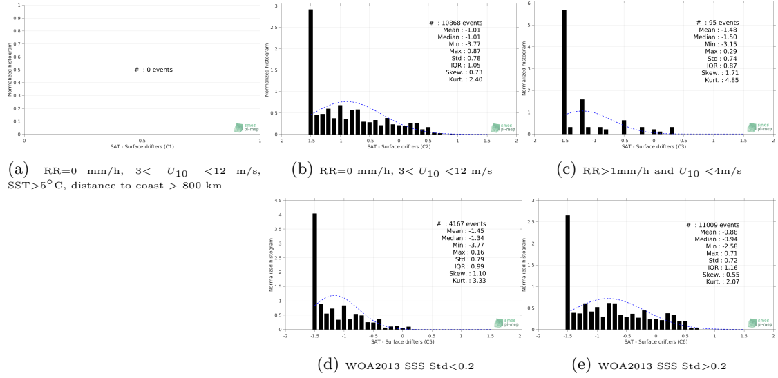
Figure 12: Normalized histogram of \Delta SSS (SMOS-L3-CATDS-CECOS-LOCEAN-V3-9DAYS-25KM - Surface drifters) for 5 different subdatasets corresponding to: RR=0 mm/h, 3 < U_{10} < 12 m/s, SST > 5°C, distance to coast > 800 km (a), RR=0 mm/h, 3 < U_{10} < 12 m/s (b), RR > 1mm/h and U_{10} < 4 m/s (c), WOA2013 SSS Std < 0.2 (d), WOA2013 SSS Std > 0.2 (e).
