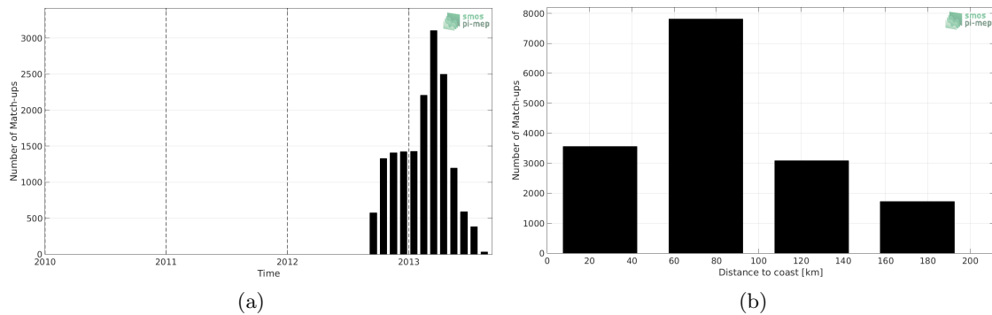
Figure 1: Number of match-ups between Surface drifters and SMOS-L3-CATDS-CECOS-LOCEAN-V3-9DAYS-25KM SSS as a function of time (a) and as function of the distance to coast (b) over the Mediterranean Sea Pi-MEP region and for the full satellite product period.
