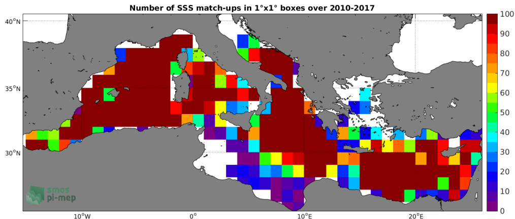
Figure 4: Number of SSS match-ups between Argo SSS and the SMOS-L3-CATDS-CECOS-LOCEAN-V3-9DAYS-25KM SSS product for the Mediterranean Sea Pi-MEP region over 1°x1° boxes and for the full satellite product period.
