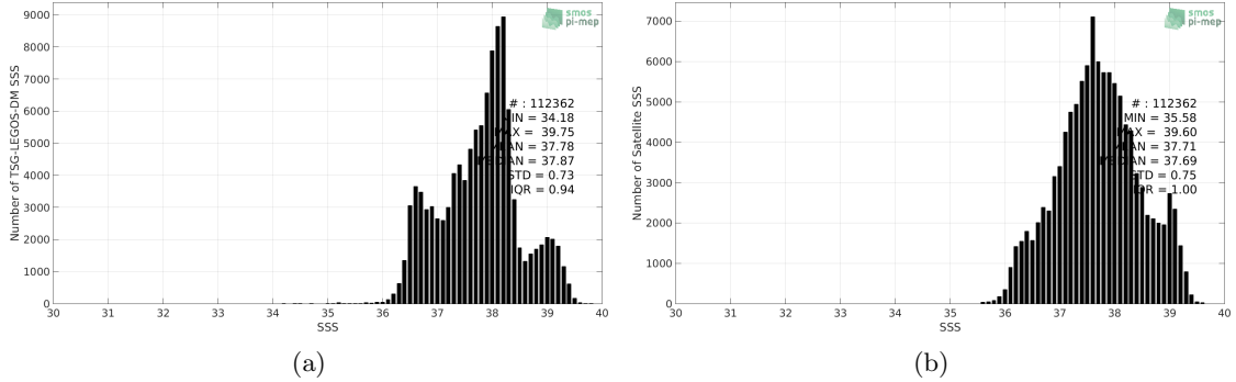
Figure 2: Histograms of SSS from TSG-LEGOS-DM (a) and SMOS-L3-CATDS-CECOS-LOCEAN-V3-18DAYS-25KM (b) considering all match-up pairs per bins of 0.1 over the Mediterranean Sea Pi-MEP region and for the full satellite product period.
