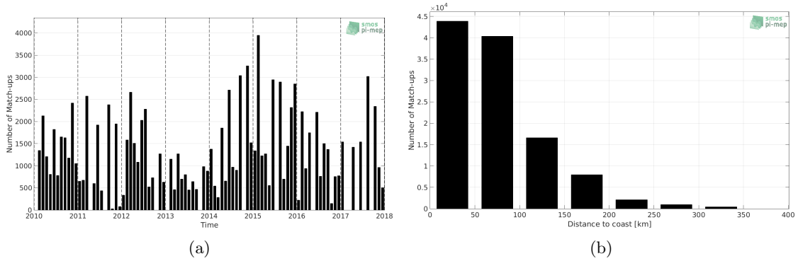
Figure 1: Number of match-ups between TSG-LEGOS-DM and SMOS-L3-CATDS-CECOS-LOCEAN-V3-18DAYS-25KM SSS as a function of time (a) and as function of the distance to coast (b) over the Mediterranean Sea Pi-MEP region and for the full satellite product period.
