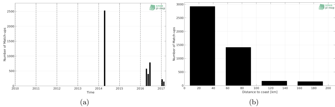
Figure 1: Number of match-ups between TSG-GOSUD-Sailing-ship and SMOS-L3-CATDS-CECOS-LOCEAN-V3-18DAYS-25KM SSS as a function of time (a) and as function of the distance to coast (b) over the Mediterranean Sea Pi-MEP region and for the full satellite product period.
