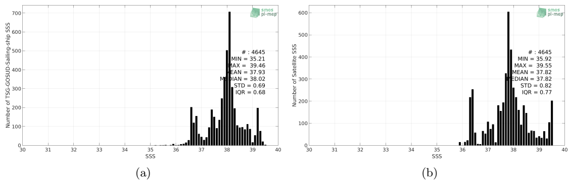
Figure 2: Histograms of SSS from TSG-GOSUD-Sailing-ship (a) and SMOS-L3-CATDS-CECOS-LOCEAN-V3-18DAYS-25KM (b) considering all match-up pairs per bins of 0.1 over the Mediterranean Sea Pi-MEP region and for the full satellite product period.
