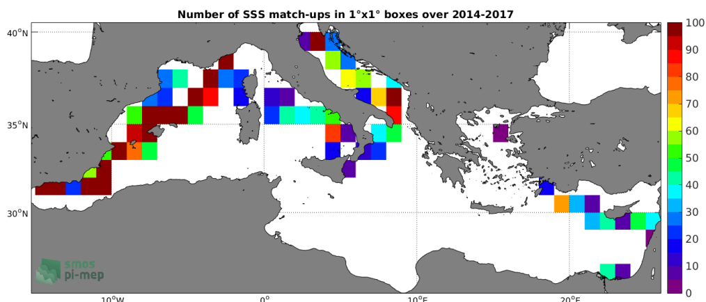
Figure 4: Number of SSS match-ups between TSG-GOSUD-Sailing-ship SSS and the SMOS-L3-CATDS-CECOS-LOCEAN-V3-18DAYS-25KM SSS product for the Mediterranean Sea Pi-MEP region over 1°x1° boxes and for the full satellite product period.
