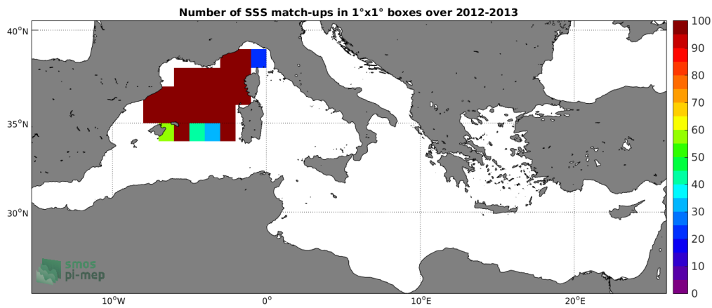
Figure 3: Number of SSS match-ups between Surface drifters SSS and the SMOS-L3-CATDS-CECOS-LOCEAN-V3-18DAYS-25KM SSS product for the Mediterranean Sea Pi-MEP region over 1°x1° boxes and for the full satellite product period.
