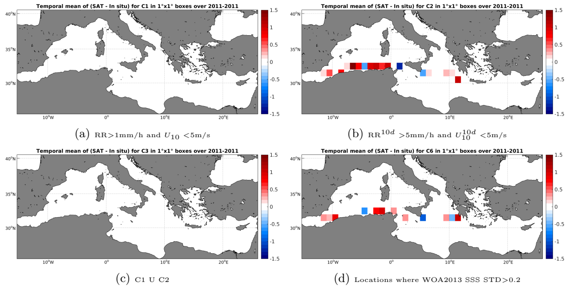
Figure 12: Temporal mean gridded over spatial boxes of size 1^\circ \times 1^\circ of \Delta SSS (SMOS-L3-CATDS-CECOS-LOCEAN-V2.1-9DAYS-25KM - TSG-SAMOS) for 4 different subdatasets corresponding to:RR > 1 mm/h and U_{10} < 5 m/s (a), RR^{10d} > 5 mm/h and U_{10}^{10d} < 5 m/s (b), C1 U C2 (c),Locations where WOA2013 SSS STD > 0.2 (d).
