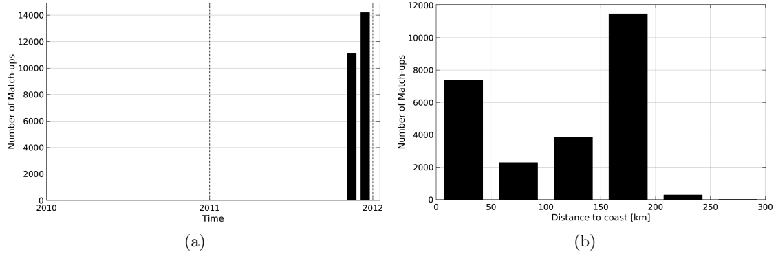
Figure 1: Number of match-ups between TSG-SAMOS and SMOS-L3-CATDS-CECOS-LOCEAN-V2.1-9DAYS-25KM SSS as a function of time (a) and as function of the distance to coast (b) over the Mediterranean Sea Pi-MEP region and for the full satellite product period.
