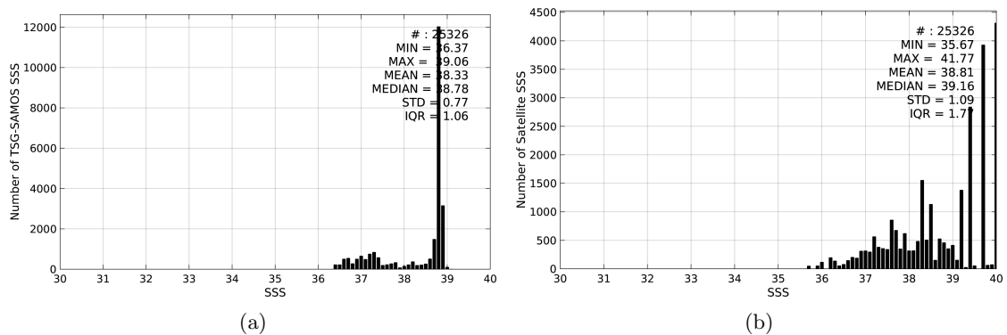
Figure 2: Histograms of SSS from TSG-SAMOS (a) and SMOS-L3-CATDS-CECOS-LOCEAN-V2.1-9DAYS-25KM (b) considering all match-up pairs per bins of 0.1 over the Mediterranean Sea Pi-MEP region and for the full satellite product period.
