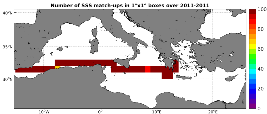
Figure 4: Number of SSS match-ups between TSG-SAMOS SSS and the SMOS-L3-CATDS-CECOS-LOCEAN-V2.1-9DAYS-25KM SSS product for the Mediterranean Sea Pi-MEP region over 1^\circ \times 1^\circ boxes and for the full satellite product period.
