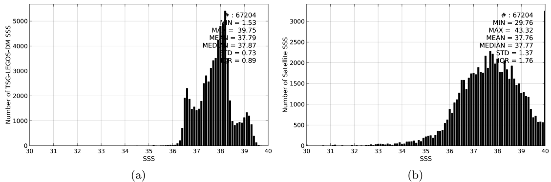
Figure 2: Histograms of SSS from TSG-LEGOS-DM (a) and SMOS-L3-CATDS-CECOS-LOCEAN-V2.1-9DAYS-25KM (b) considering all match-up pairs per bins of 0.1 over the Mediterranean Sea Pi-MEP region and for the full satellite product period.
