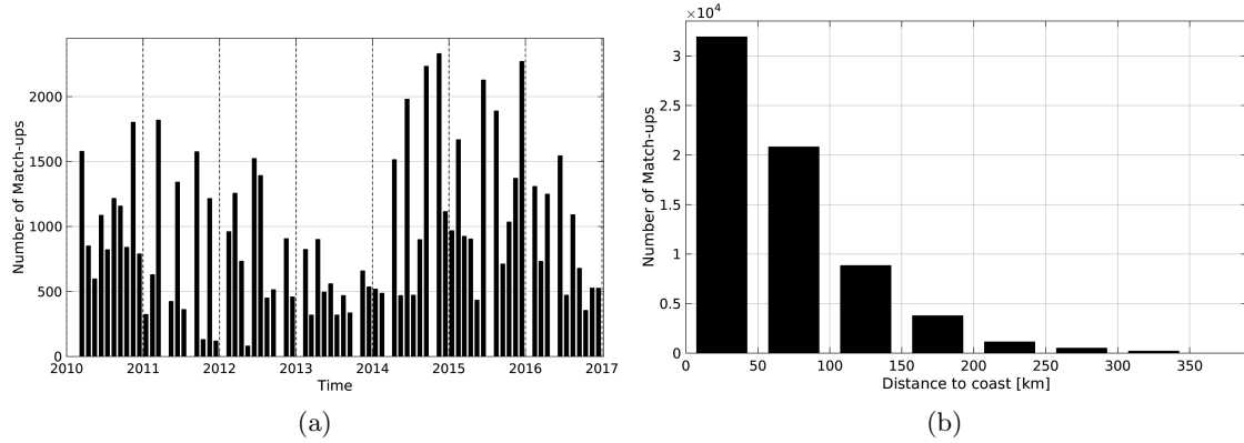
Figure 1: Number of match-ups between TSG-LEGOS-DM and SMOS-L3-CATDS-CECOS-LOCEAN-V2.1-9DAYS-25KM SSS as a function of time (a) and as function of the distance to coast (b) over the Mediterranean Sea Pi-MEP region and for the full satellite product period.
