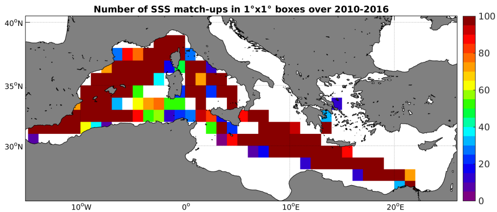
Figure 4: Number of SSS match-ups between TSG-LEGOS-DM SSS and the SMOS-L3-CATDS-CECOS-LOCEAN-V2.1-9DAYS-25KM SSS product for the Mediterranean Sea Pi-MEP region over 1^\circ \times 1^\circ boxes and for the full satellite product period.
