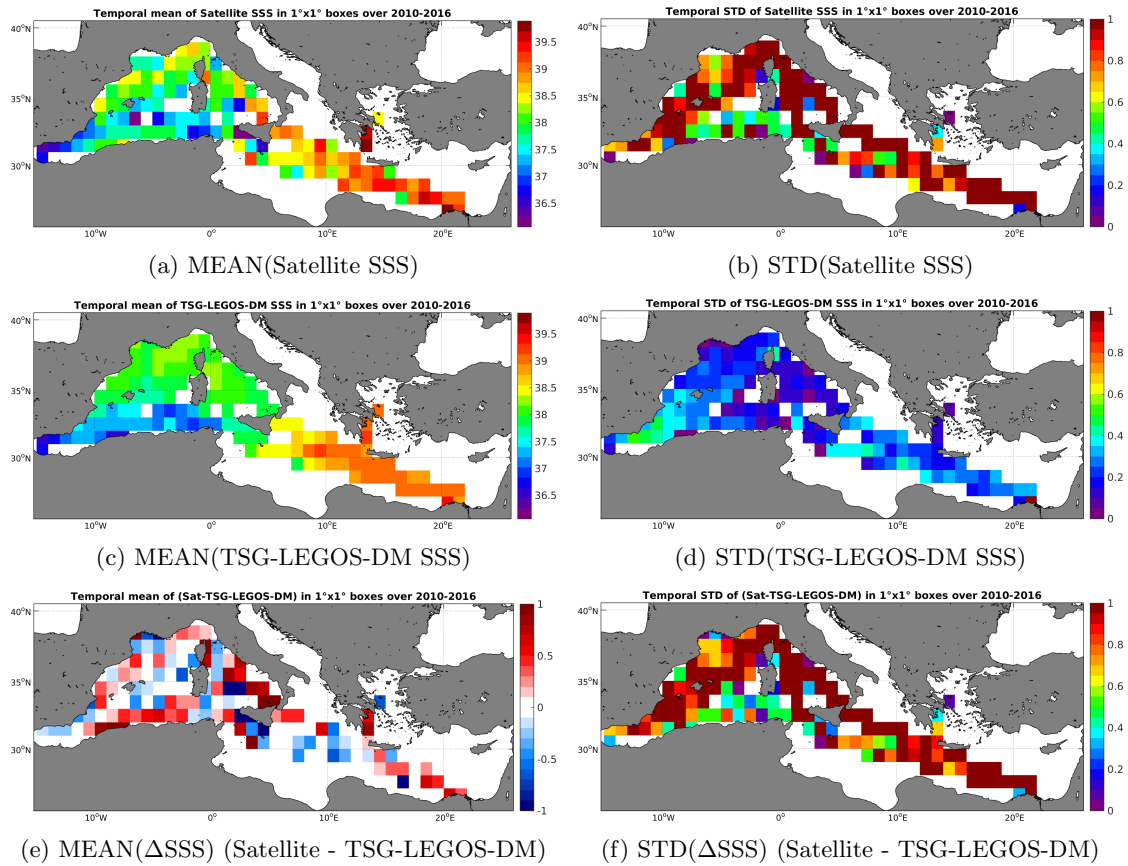
Figure 6: Temporal mean (left) and STD (right) of SSS from SMOS-L3-CATDS-CECOS-LOCEAN-V2.1-9DAYS-25KM (top), TSG-LEGOS-DM (middle), and of \Delta SSS (Satellite - TSG-LEGOS-DM). Only match-up pairs are used to generate these maps.
