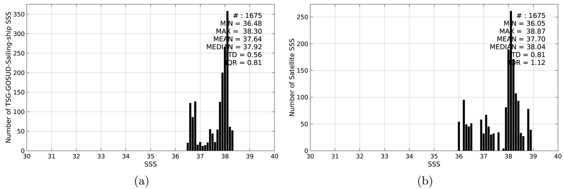
Figure 2: Histograms of SSS from TSG-GOSUD-Sailing-ship (a) and SMOS-L3-CATDS-CECOS-LOCEAN-V2.1-9DAYS-25KM (b) considering all match-up pairs per bins of 0.1 over the Mediterranean Sea Pi-MEP region and for the full satellite product period.
