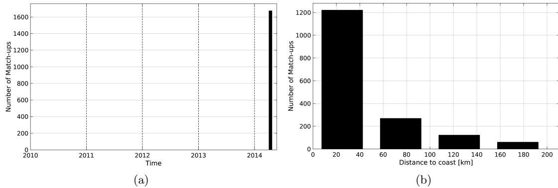
Figure 1: Number of match-ups between TSG-GOSUD-Sailing-ship and SMOS-L3-CATDS-CECOS-LOCEAN-V2.1-9DAYS-25KM SSS as a function of time (a) and as function of the distance to coast (b) over the Mediterranean Sea Pi-MEP region and for the full satellite product period.
