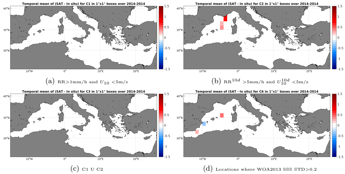
Figure 12: Temporal mean gridded over spatial boxes of size 1^\circ \times 1^\circ of \Delta SSS (SMOS-L3-CATDS-CECOS-LOCEAN-V2.1-9DAYS-25KM - TSG-GOSUD-Sailing-ship) for 4 different subdatasets corresponding to: RR > 1mm/h and U_{10} < 5\text{m/s} (a), RR^{10d} > 5\text{mm/h} and U_{10}^{10d} < 5\text{m/s} (b), C1 U C2 (c), Locations where WOA2013 SSS STD > 0.2 (d).
