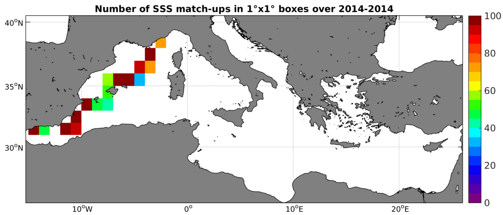
Figure 4: Number of SSS match-ups between TSG-GOSUD-Sailing-ship SSS and the SMOS-L3-CATDS-CECOS-LOCEAN-V2.1-9DAYS-25KM SSS product for the Mediterranean Sea Pi-MEP region over 1^\circ \times 1^\circ boxes and for the full satellite product period.
