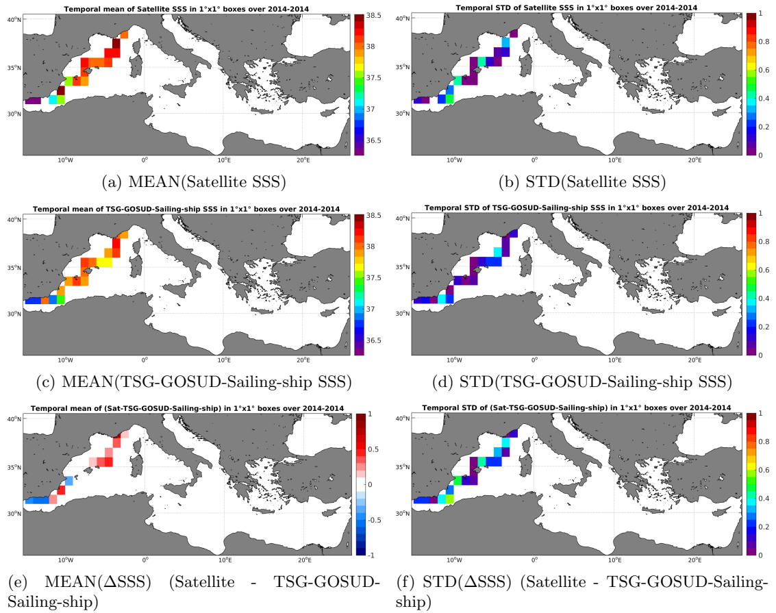
Figure 6: Temporal mean (left) and STD (right) of SSS from SMOS-L3-CATDS-CECOS-LOCEAN-V2.1-9DAYS-25KM (top), TSG-GOSUD-Sailing-ship (middle), and of \Delta SSS (Satellite - TSG-GOSUD-Sailing-ship). Only match-up pairs are used to generate these maps.
