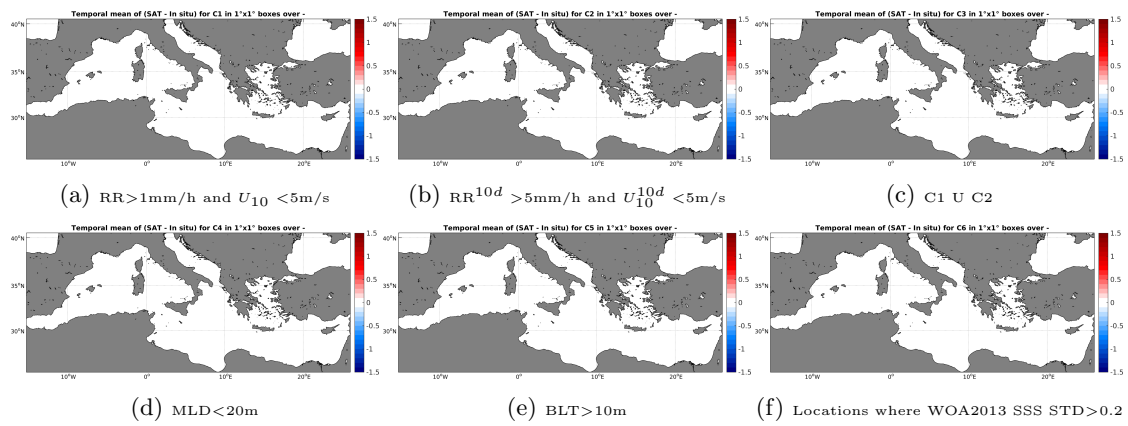
Figure 12: Temporal mean gridded over spatial boxes of size 1^\circ \times 1^\circ of \Delta SSS (SMOS-L3-CATDS-CECOS-LOCEAN-V2.1-9DAYS-25KM - Sea mammals) for 6 different subdatasets corresponding to: RR > 1\text{mm/h} and U_{10} < 5\text{m/s} (a), RR^{10d} > 5\text{mm/h} and U_{10}^{10d} < 5\text{m/s} (b), C1 U C2 (c), MLD < 20\text{m} (d), BLT > 10\text{m} (e), Locations where WOA2013 SSS STD > 0.2 (f).
