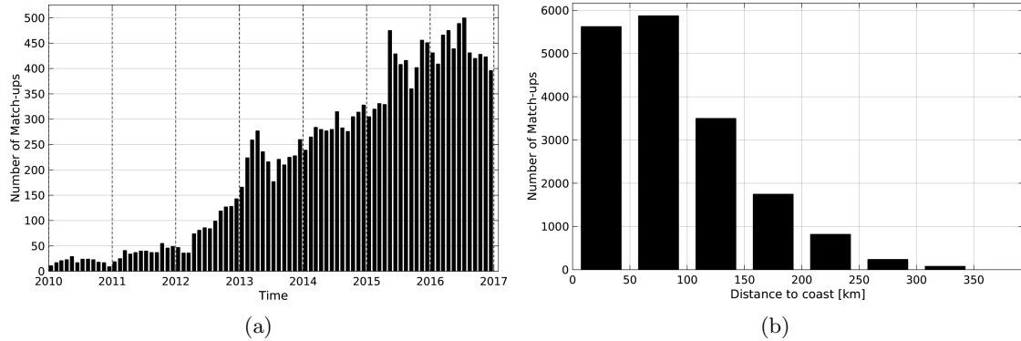
Figure 1: Number of match-ups between Argo and SMOS-L3-CATDS-CECOS-LOCEAN-V2.1-9DAYS-25KM SSS as a function of time (a) and as function of the distance to coast (b) over the Mediterranean Sea Pi-MEP region and for the full satellite product period.
