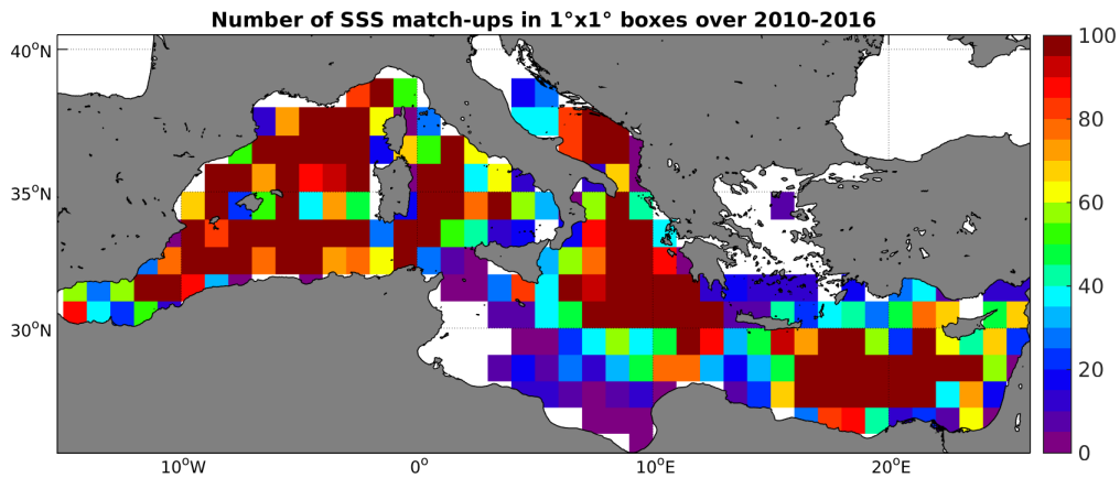
Figure 4: Number of SSS match-ups between Argo SSS and the SMOS-L3-CATDS-CECOS-LOCEAN-V2.1-9DAYS-25KM SSS product for the Mediterranean Sea Pi-MEP region over 1^\circ \times 1^\circ boxes and for the full satellite product period.
