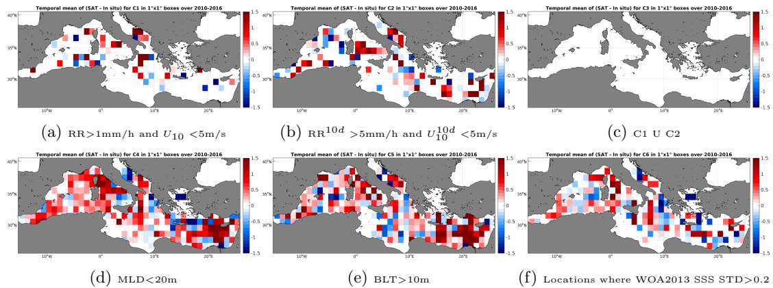
Figure 12: Temporal mean gridded over spatial boxes of size 1^\circ \times 1^\circ of \Delta SSS (SMOS-L3-CATDS-CECOS-LOCEAN-V2.1-9DAYS-25KM - Argo) for 6 different subdatasets corresponding to:RR >1 mm/h and U_{10} < 5 m/s (a), RR ^{10d} > 5 mm/h and U_{10}^{10d} < 5 m/s (b), C1 U C2 (c),MLD <20 m (d),BLT >10 m (e),Locations where WOA2013 SSS STD >0.2 (f).
