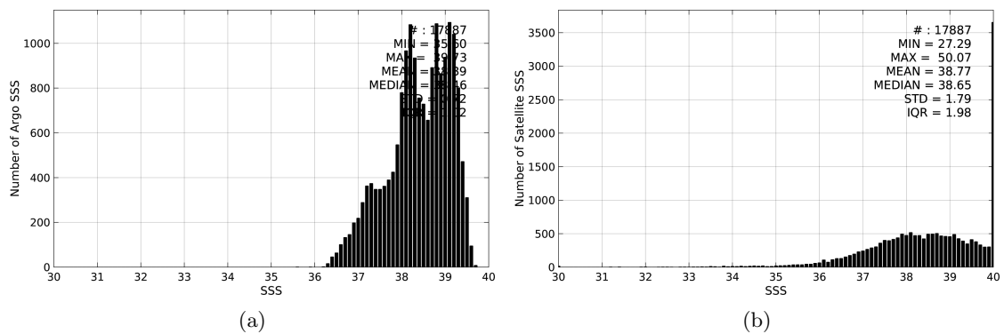
Figure 2: Histograms of SSS from Argo (a) and SMOS-L3-CATDS-CECOS-LOCEAN-V2.1-9DAYS-25KM (b) considering all match-up pairs per bins of 0.1 over the Mediterranean Sea Pi-MEP region and for the full satellite product period.
