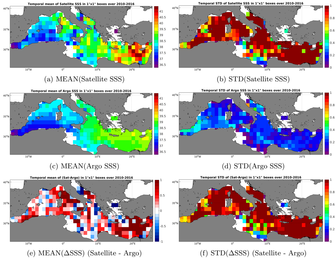
Figure 6: Temporal mean (left) and STD (right) of SSS from SMOS-L3-CATDS-CECOS-LOCEAN-V2.1-9DAYS-25KM (top), Argo (middle), and of \Delta SSS (Satellite - Argo). Only match-up pairs are used to generate these maps.
