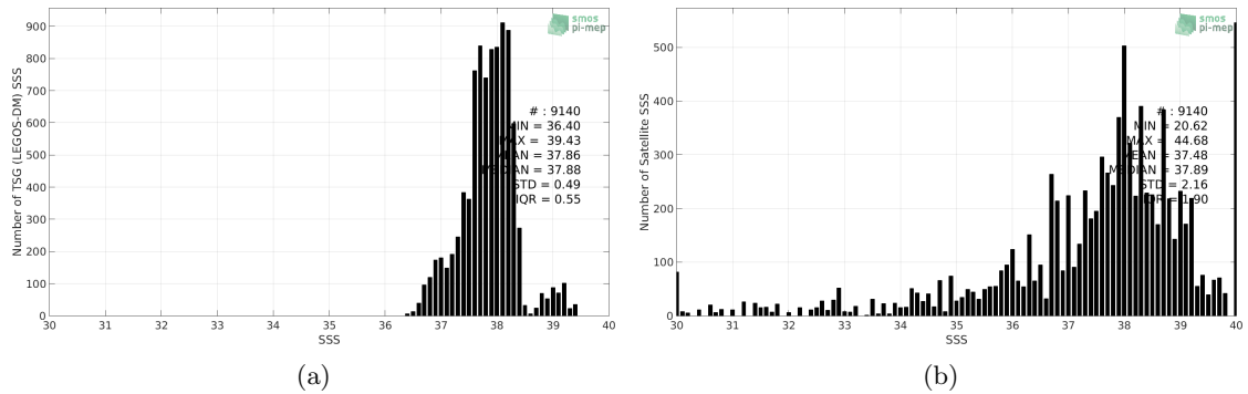
Figure 2: Histograms of SSS from TSG (LEGOS-DM) (a) and SMOS SSS L3 v2 - Monthly - 0.25 Deg (CATDS-CECOS-IFREMER) (b) considering all match-up pairs per bins of 0.1 over the Mediterranean Sea Pi-MEP region and for the full satellite product period.
