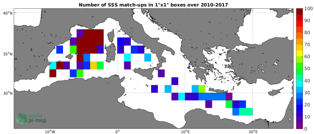
Figure 4: Number of SSS match-ups between TSG (LEGOS-DM) SSS and the SMOS SSS L3 v2 - Monthly - 0.25 Deg (CATDS-CECOS-IFREMER) SSS product for the Mediterranean Sea Pi-MEP region over 1^\circ \times 1^\circ boxes and for the full satellite product period.
