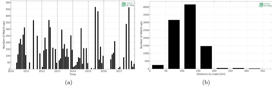
Figure 1: Number of match-ups between TSG (LEGOS-DM) and SMOS SSS L3 v2 - Monthly - 0.25 Deg (CATDS-CECOS-IFREMER) SSS as a function of time (a) and as function of the distance to coast (b) over the Mediterranean Sea Pi-MEP region and for the full satellite product period.
