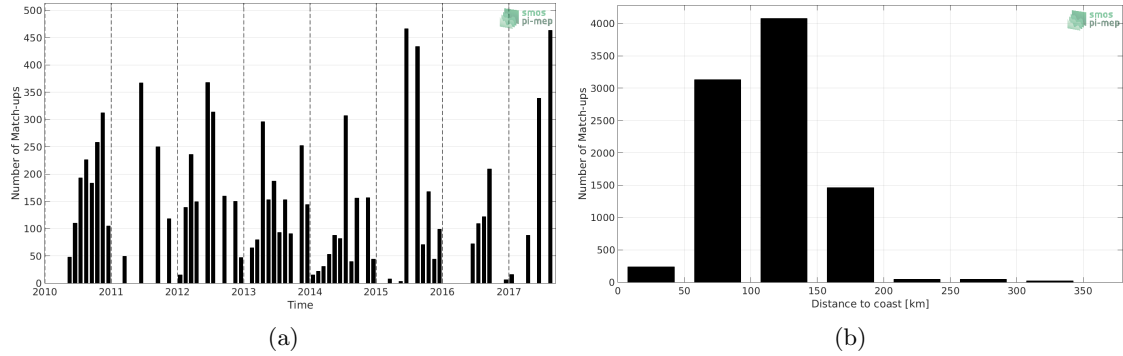
Figure 1: Number of match-ups between TSG-LEGOS-DM and SMOS L3 v2 - Monthly - 0.25 Deg (CATDS-CECOS-IFREMER) SSS as a function of time (a) and as function of the distance to coast (b) over the Mediterranean Sea Pi-MEP region and for the full satellite product period.
