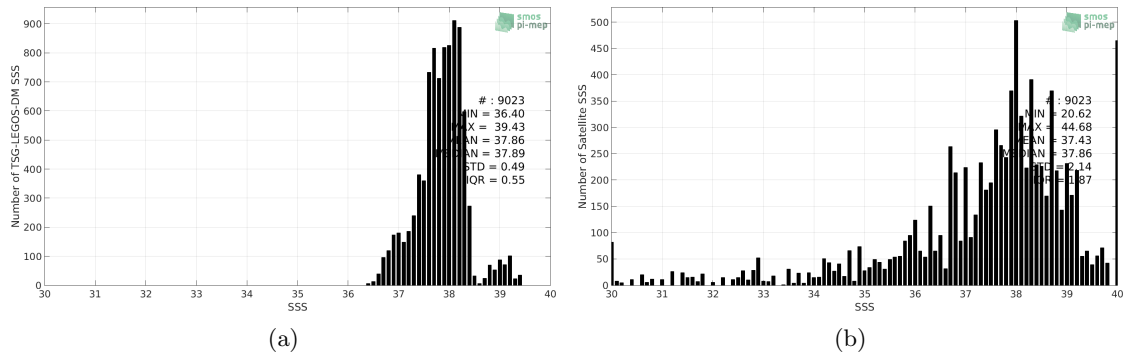
Figure 2: Histograms of SSS from TSG-LEGOS-DM (a) and SMOS L3 v2 - Monthly - 0.25 Deg (CATDS-CECOS-IFREMER) (b) considering all match-up pairs per bins of 0.1 over the Mediterranean Sea Pi-MEP region and for the full satellite product period.
