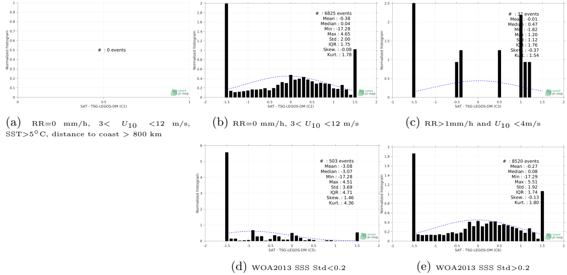
Figure 13: Normalized histogram of \Delta SSS (SMOS L3 v2 - Monthly - 0.25 Deg (CATDS-CECOS-IFREMER) - TSG-LEGOS-DM) for 5 different subdatasets corresponding to: RR=0 mm/h, 3 < U_{10} < 12 m/s, SST>5°C, distance to coast > 800 km (a), RR=0 mm/h, 3 < U_{10} < 12 m/s (b), RR>1mm/h and U_{10} < 4 m/s (c), WOA2013 SSS Std<0.2 (d), WOA2013 SSS Std>0.2 (e).
