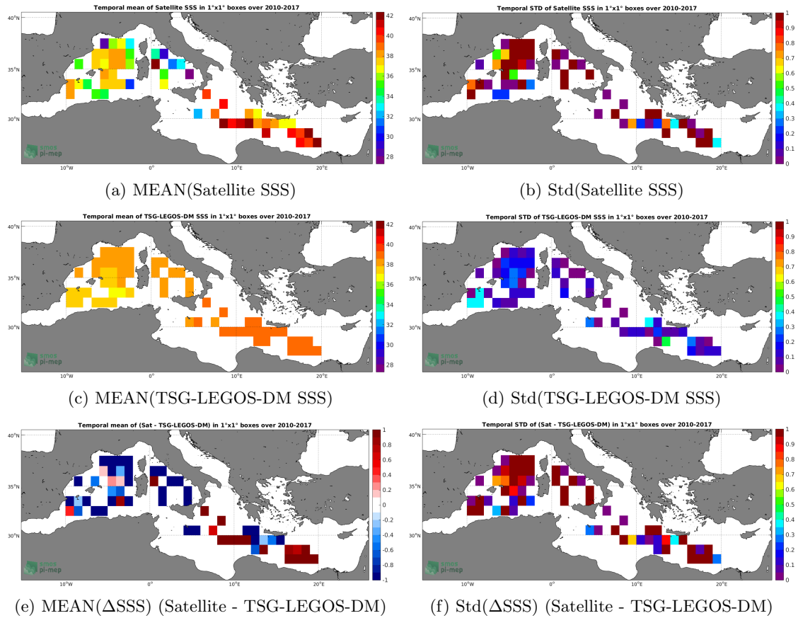
Figure 6: Temporal mean (left) and Std (right) of SSS from SMOS L3 v2 - Monthly - 0.25 Deg (CATDS-CECOS-IFREMER) (top), TSG-LEGOS-DM (middle), and of \Delta SSS (Satellite - TSG-LEGOS-DM). Only match-up pairs are used to generate these maps.
