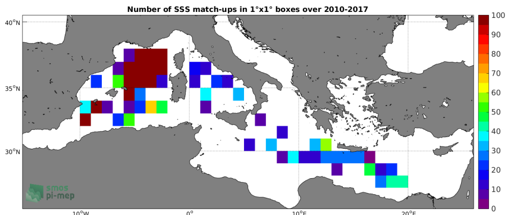
Figure 4: Number of SSS match-ups between TSG-LEGOS-DM SSS and the SMOS L3 v2 - Monthly - 0.25 Deg (CATDS-CECOS-IFREMER) SSS product for the Mediterranean Sea Pi-MEP region over 1^\circ \times 1^\circ boxes and for the full satellite product period.
