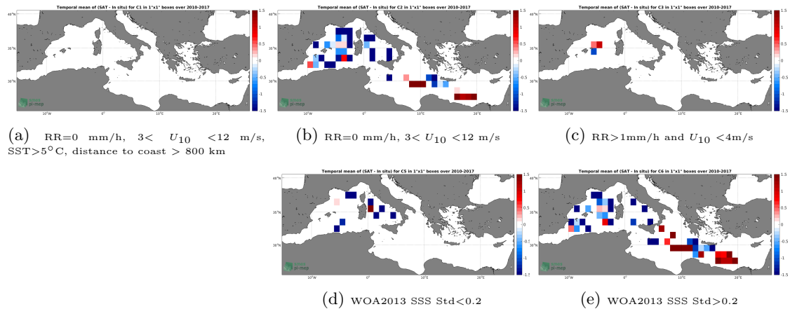
Figure 12: Temporal mean gridded over spatial boxes of size 1^{\circ}\times 1^{\circ} of \Delta\text{SSS} (SMOS L3 v2 - Monthly - 0.25 Deg (CATDS-CECOS-IFREMER) - TSG-LEGOS-DM) for 5 different subdatasets corresponding to:RR=0 mm/h, 3 < U_{10} < 12 m/s, SST > 5^{\circ}\text{C} , distance to coast > 800 km (a), RR=0 mm/h, 3 < U_{10} < 12 m/s (b), RR > 1 mm/h and U_{10} < 4 m/s (c), WOA2013 SSS Std < 0.2 (d), WOA2013 SSS Std > 0.2 (e).
