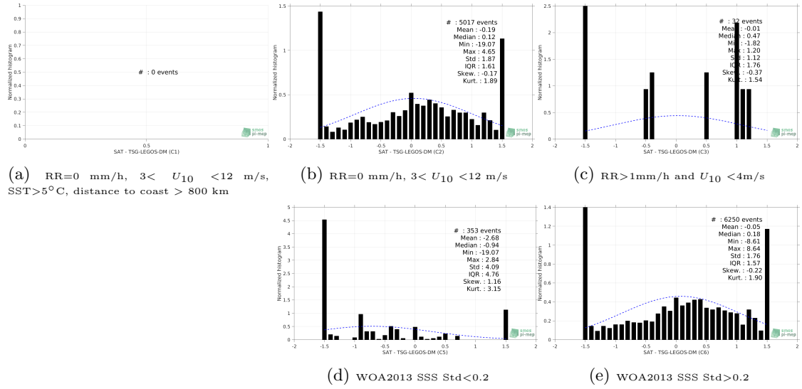
Figure 13: Normalized histogram of \Delta SSS (SMOS-L3-CATDS-IFREMER-CECOS-V2-MONTHLY-0.25DEG - TSG-LEGOS-DM) for 5 different subdatasets corresponding to: RR=0 mm/h, 3 < U_{10} < 12 m/s, SST > 5°C, distance to coast > 800 km (a), RR=0 mm/h, 3 < U_{10} < 12 m/s (b), RR > 1mm/h and U_{10} < 4 m/s (c), WOA2013 SSS Std < 0.2 (d), WOA2013 SSS Std > 0.2 (e).
