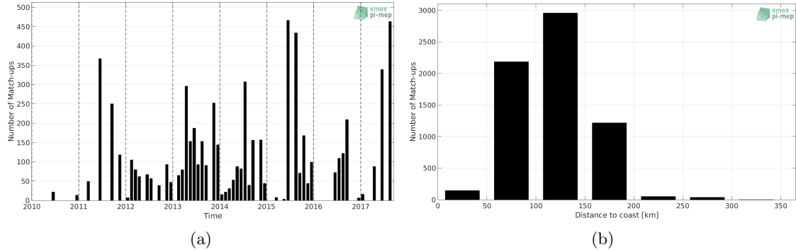
Figure 1: Number of match-ups between TSG-LEGOS-DM and SMOS-L3-CATDS-IFREMER-CECOS-V2-MONTHLY-0.25DEG SSS as a function of time (a) and as function of the distance to coast (b) over the Mediterranean Sea Pi-MEP region and for the full satellite product period.
