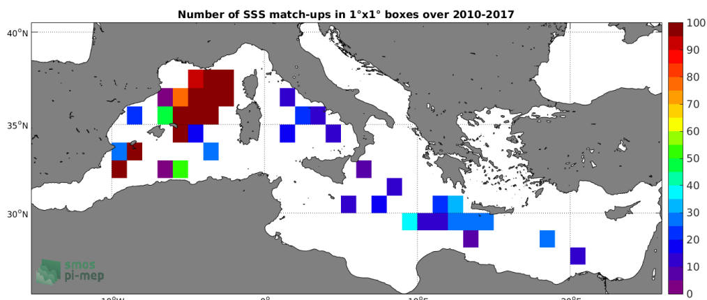
Figure 4: Number of SSS match-ups between TSG-LEGOS-DM SSS and the SMOS-L3-CATDS-IFREMER-CECOS-V2-MONTHLY-0.25DEG SSS product for the Mediterranean Sea Pi-MEP region over 1^\circ \times 1^\circ boxes and for the full satellite product period.
