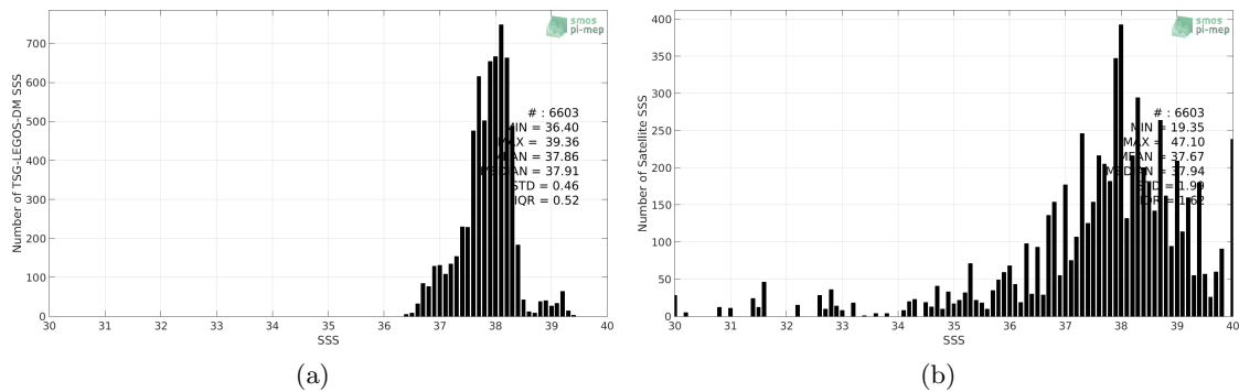
Figure 2: Histograms of SSS from TSG-LEGOS-DM (a) and SMOS-L3-CATDS-IFREMER-CECOS-V2-MONTHLY-0.25DEG (b) considering all match-up pairs per bins of 0.1 over the Mediterranean Sea Pi-MEP region and for the full satellite product period.
