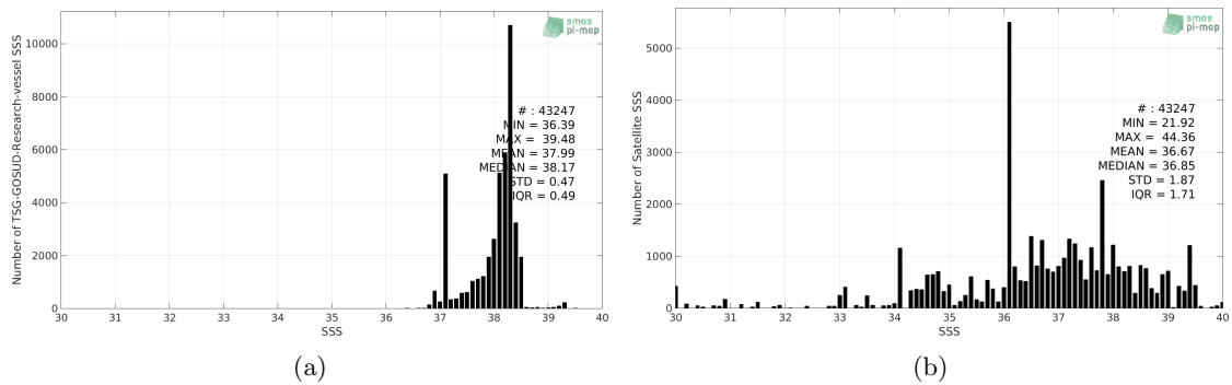
Figure 2: Histograms of SSS from TSG-GOSUD-Research-vessel (a) and SMOS-L3-CATDS-IFREMER-CECOS-V2-MONTHLY-0.25DEG (b) considering all match-up pairs per bins of 0.1 over the Mediterranean Sea Pi-MEP region and for the full satellite product period.
