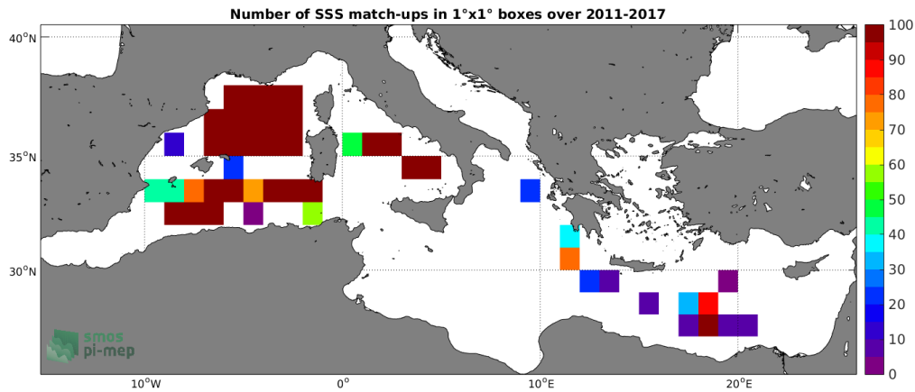
Figure 4: Number of SSS match-ups between TSG-GOSUD-Research-vessel SSS and the SMOS-L3-CATDS-IFREMER-CECOS-V2-MONTHLY-0.25DEG SSS product for the Mediterranean Sea Pi-MEP region over 1°x1° boxes and for the full satellite product period.
