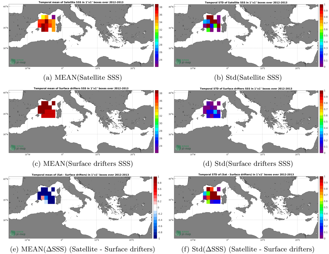
Figure 5: Temporal mean (left) and Std (right) of SSS from SMOS SSS L3 v2 - Monthly - 0.25 Deg (CATDS-CECOS-IFREMER) (top), Surface drifters (middle), and of \Delta SSS (Satellite - Surface drifters). Only match-up pairs are used to generate these maps.
