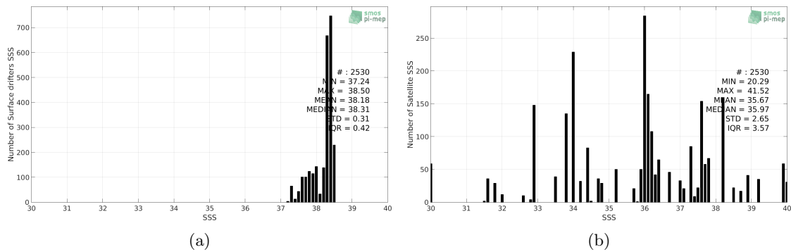
Figure 2: Histograms of SSS from Surface drifters (a) and SMOS SSS L3 v2 - Monthly - 0.25 Deg (CATDS-CECOS-IFREMER) (b) considering all match-up pairs per bins of 0.1 over the Mediterranean Sea Pi-MEP region and for the full satellite product period.
