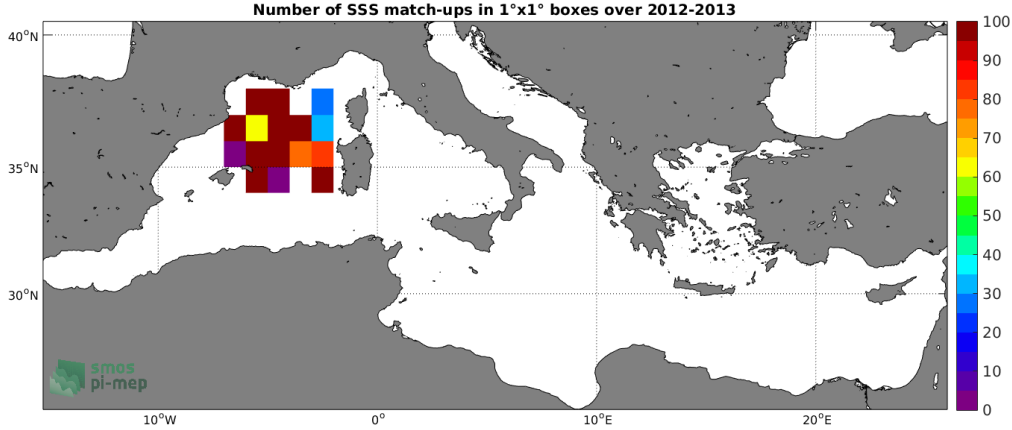
Figure 3: Number of SSS match-ups between Surface drifters SSS and the SMOS SSS L3 v2 - Monthly - 0.25 Deg (CATDS-CECOS-IFREMER) SSS product for the Mediterranean Sea Pi-MEP region over 1^\circ \times 1^\circ boxes and for the full satellite product period.
