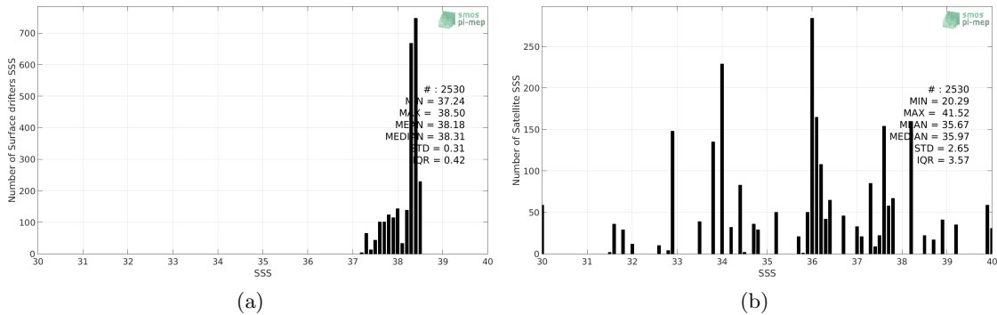
Figure 2: Histograms of SSS from Surface drifters (a) and SMOS L3 v2 - Monthly - 0.25 Deg (CATDS-CECOS-IFREMER) (b) considering all match-up pairs per bins of 0.1 over the Mediterranean Sea Pi-MEP region and for the full satellite product period.
