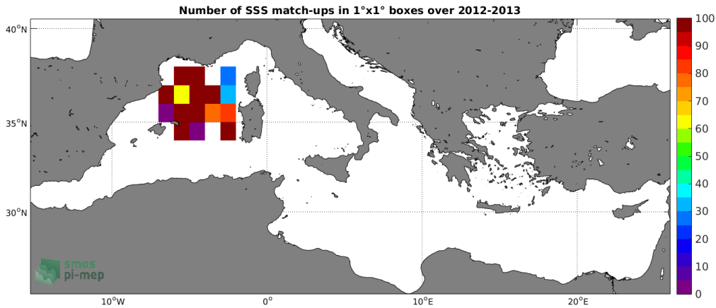
Figure 3: Number of SSS match-ups between Surface drifters SSS and the SMOS L3 v2 - Monthly - 0.25 Deg (CATDS-CECOS-IFREMER) SSS product for the Mediterranean Sea Pi-MEP region over 1^\circ \times 1^\circ boxes and for the full satellite product period.
