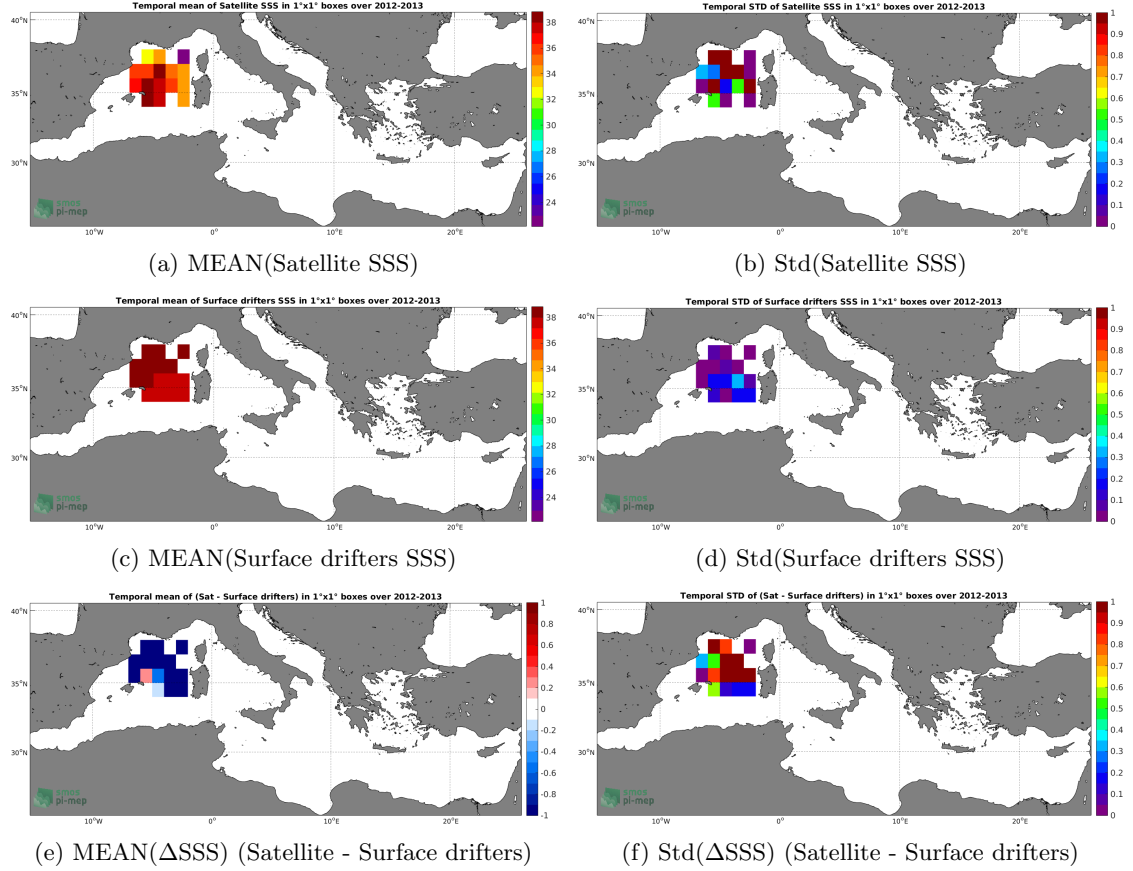
Figure 5: Temporal mean (left) and Std (right) of SSS from SMOS L3 v2 - Monthly - 0.25 Deg (CATDS-CECOS-IFREMER) (top), Surface drifters (middle), and of \Delta SSS (Satellite - Surface drifters). Only match-up pairs are used to generate these maps.
