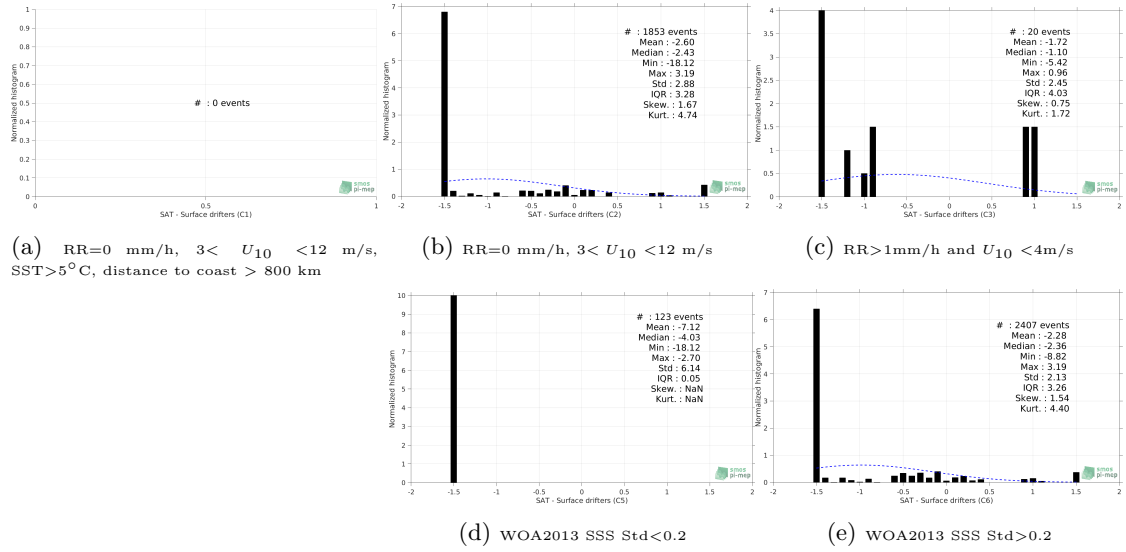
Figure 12: Normalized histogram of \Delta SSS (SMOS L3 v2 - Monthly - 0.25 Deg (CATDS-CECOS-IFREMER) - Surface drifters) for 5 different subdatasets corresponding to: RR=0 mm/h, 3 < U_{10} < 12 m/s, SST > 5°C, distance to coast > 800 km (a), RR=0 mm/h, 3 < U_{10} < 12 m/s (b), RR > 1mm/h and U_{10} < 4 m/s (c), WOA2013 SSS Std < 0.2 (d), WOA2013 SSS Std > 0.2 (e).
