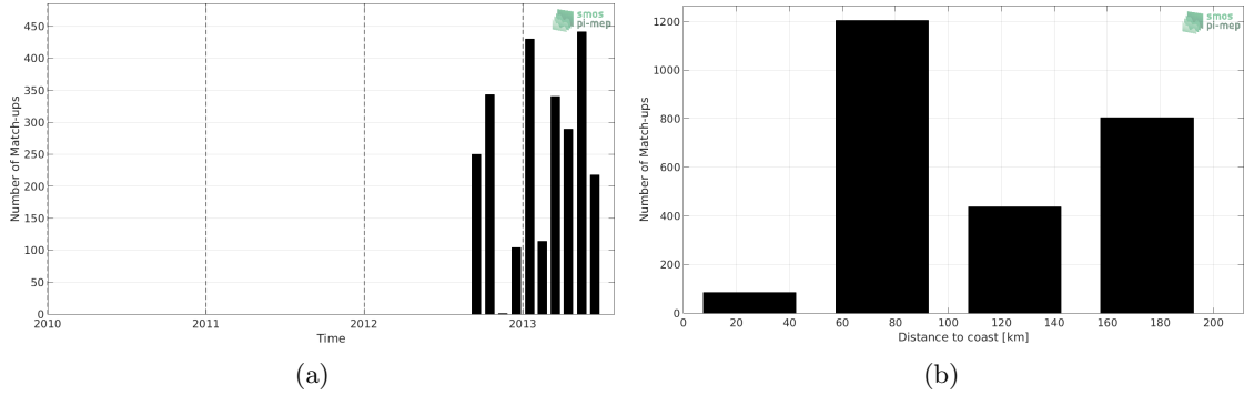
Figure 1: Number of match-ups between Surface drifters and SMOS L3 v2 - Monthly - 0.25 Deg (CATDS-CECOS-IFREMER) SSS as a function of time (a) and as function of the distance to coast (b) over the Mediterranean Sea Pi-MEP region and for the full satellite product period.
