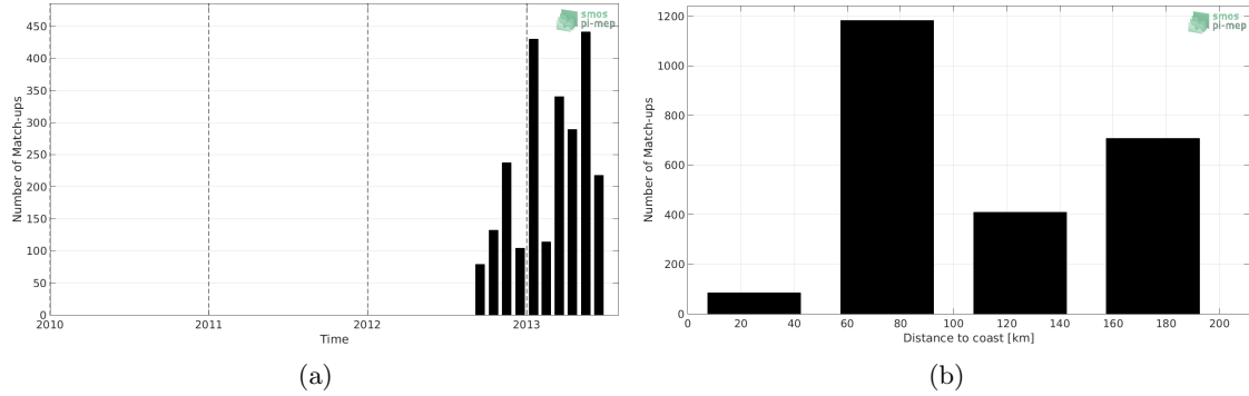
Figure 1: Number of match-ups between Surface drifters and SMOS-L3-CATDS-IFREMER-CECOS-V2-MONTHLY-0.25DEG SSS as a function of time (a) and as function of the distance to coast (b) over the Mediterranean Sea Pi-MEP region and for the full satellite product period.
