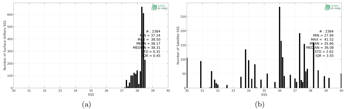
Figure 2: Histograms of SSS from Surface drifters (a) and SMOS-L3-CATDS-IFREMER-CECOS-V2-MONTHLY-0.25DEG (b) considering all match-up pairs per bins of 0.1 over the Mediterranean Sea Pi-MEP region and for the full satellite product period.
