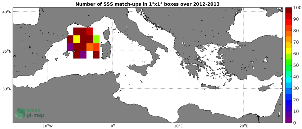
Figure 3: Number of SSS match-ups between Surface drifters SSS and the SMOS-L3-CATDS-IFREMER-CECOS-V2-MONTHLY-0.25DEG SSS product for the Mediterranean Sea Pi-MEP region over 1^\circ \times 1^\circ boxes and for the full satellite product period.
