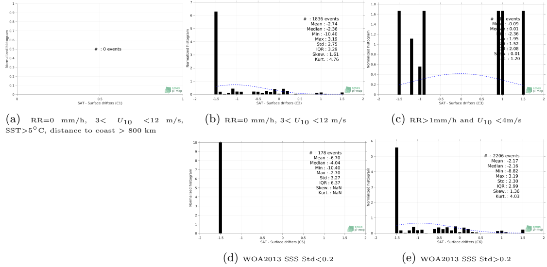
Figure 12: Normalized histogram of \Delta SSS (SMOS-L3-CATDS-IFREMER-CECOS-V2-MONTHLY-0.25DEG - Surface drifters) for 5 different subdatasets corresponding to: RR=0 mm/h, 3 < U_{10} < 12 m/s, SST > 5°C, distance to coast > 800 km (a), RR=0 mm/h, 3 < U_{10} < 12 m/s (b), RR > 1mm/h and U_{10} < 4 m/s (c), WOA2013 SSS Std < 0.2 (d), WOA2013 SSS Std > 0.2 (e).
