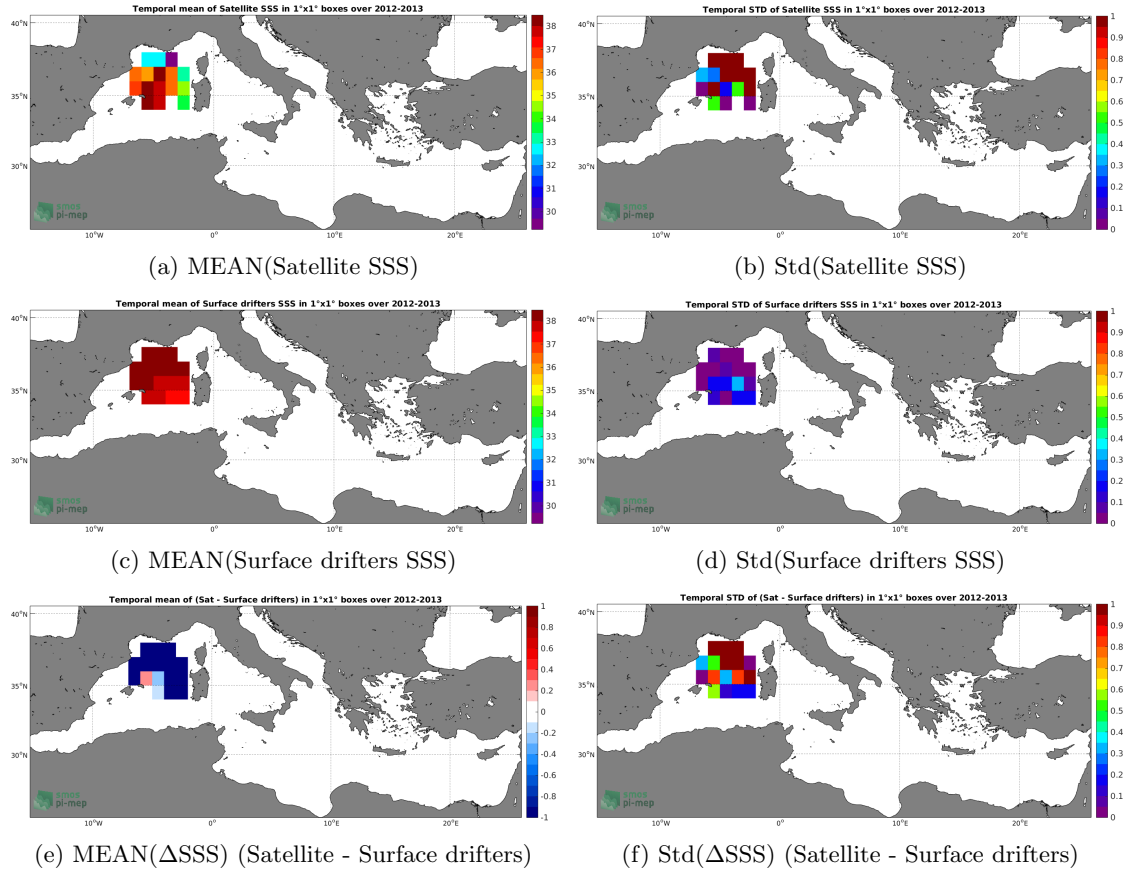
Figure 5: Temporal mean (left) and Std (right) of SSS from SMOS-L3-CATDS-IFREMER-CECOS-V2-MONTHLY-0.25DEG (top), Surface drifters (middle), and of \Delta SSS (Satellite - Surface drifters). Only match-up pairs are used to generate these maps.
