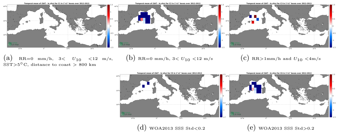
Figure 11: Temporal mean gridded over spatial boxes of size 1^\circ \times 1^\circ of \Delta SSS (SMOS-L3-CATDS-IFREMER-CECOS-V2-MONTHLY-0.25DEG - Surface drifters) for 5 different subdatasets corresponding to:RR=0 mm/h, 3 < U_{10} < 12 m/s, SST >5^\circ C, distance to coast > 800 km (a), RR=0 mm/h, 3 < U_{10} < 12 m/s (b), RR >1 mm/h and U_{10} < 4 m/s (c), WOA2013 SSS Std <0.2 (d), WOA2013 SSS Std >0.2 (e).
