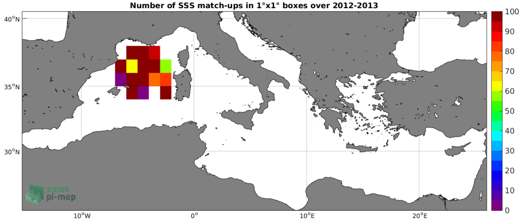
Figure 3: Number of SSS match-ups between Surface drifters SSS and the SMOS-L3-CATDS-IFREMER-CECOS-V2-MONTHLY-0.25DEG SSS product for the Mediterranean Sea Pi-MEP region over 1°x1° boxes and for the full satellite product period.
