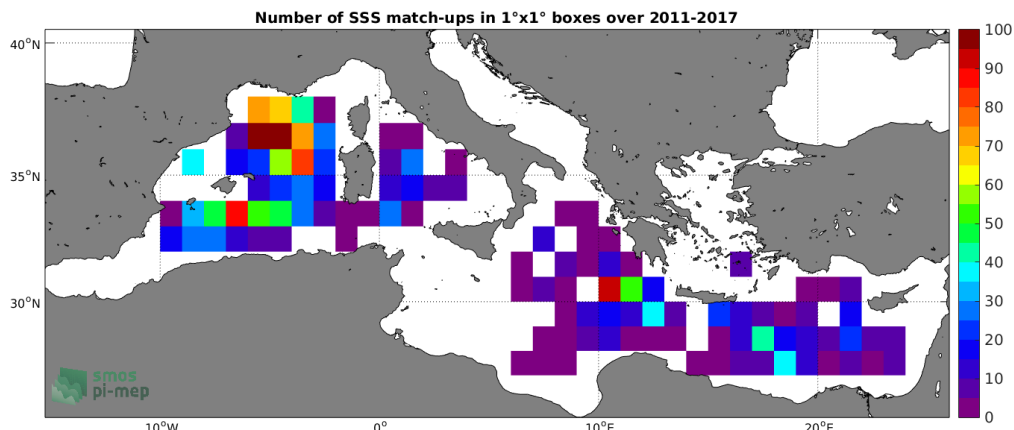
Figure 4: Number of SSS match-ups between Argo SSS and the SMOS-L3-CATDS-IFREMER-CECOS-V2-MONTHLY-0.25DEG SSS product for the Mediterranean Sea Pi-MEP region over 1^\circ \times 1^\circ boxes and for the full satellite product period.
