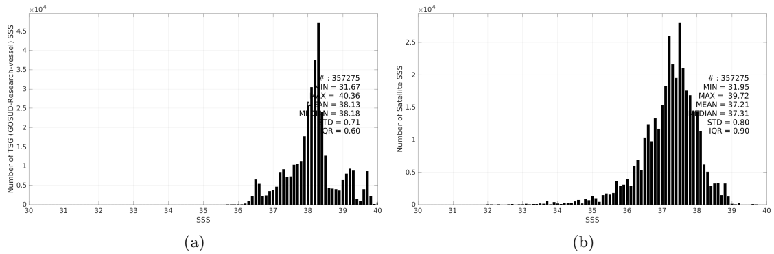
Figure 3: Histograms of SSS from TSG (GOSUD-Research-vessel) (a) and SMOS SSS L3 v335 - Monthly - 25 km (CATDS-CPDC) (b) considering all match-up pairs per bins of 0.1 over the Mediterranean Sea Pi-MEP region and for the full satellite product period.
