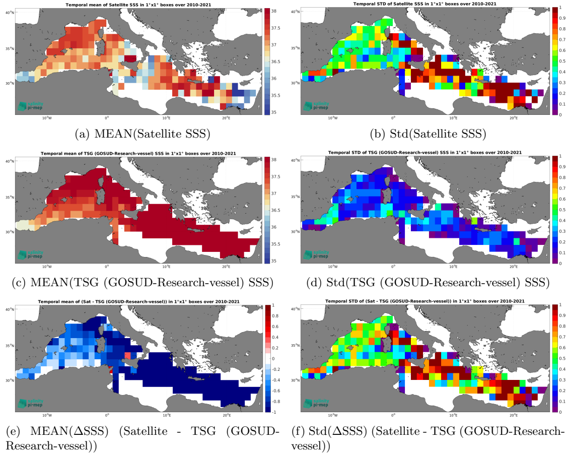
Figure 7: Temporal mean (left) and Std (right) of SSS from SMOS SSS L3 v335 - Monthly - 25 km (CATDS-CPDC) (top), TSG (GOSUD-Research-vessel) ( in situ ) (middle), and of \Delta\text{SSS} (Satellite - TSG (GOSUD-Research-vessel)). Only match-up pairs are used to generate these maps.
