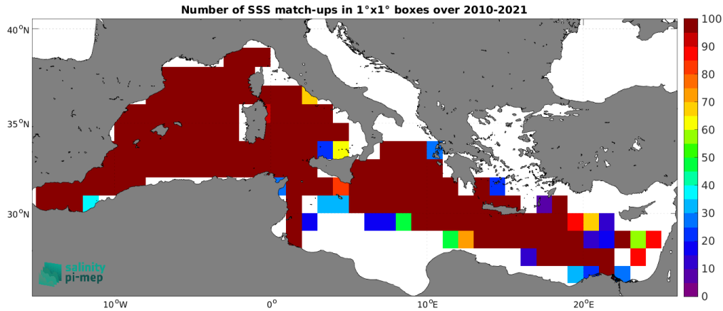
Figure 5: Number of SSS match-ups between TSG (GOSUD-Research-vessel) SSS and the SMOS SSS L3 v335 - Monthly - 25 km (CATDS-CPDC) SSS product for the Mediterranean Sea Pi-MEP region over 1^\circ \times 1^\circ boxes and for the full satellite product period.
