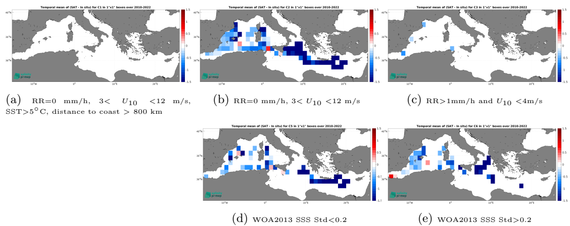
Figure 14: Temporal mean gridded over spatial boxes of size 1^\circ \times 1^\circ of \Delta\text{SSS} (SMOS SSS L3 v335 - Monthly - 25 km (CATDS-CPDC) - TSG (CSIC-UTM)) for 5 different subdatasets corresponding to:RR=0 mm/h, 3 < U_{10} < 12 m/s, SST>5°C, distance to coast > 800 km (a), RR=0 mm/h, 3 < U_{10} < 12 m/s (b), RR>1mm/h and U_{10} < 4 m/s (c), WOA2013 SSS Std<0.2 (d), WOA2013 SSS Std>0.2 (e).
