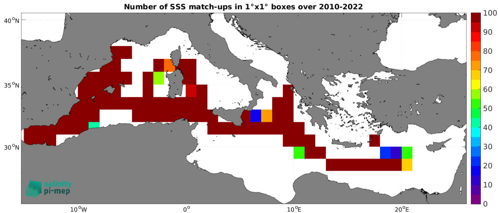
Figure 5: Number of SSS match-ups between TSG (CSIC-UTM) SSS and the SMOS SSS L3 v335 - Monthly - 25 km (CATDS-CPDC) SSS product for the Mediterranean Sea Pi-MEP region over 1^\circ \times 1^\circ boxes and for the full satellite product period.
