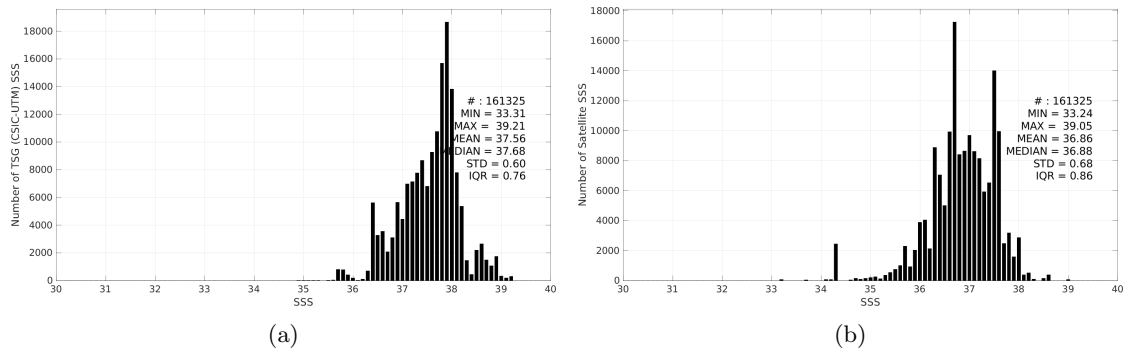
Figure 3: Histograms of SSS from TSG (CSIC-UTM) (a) and SMOS SSS L3 v335 - Monthly - 25 km (CATDS-CPDC) (b) considering all match-up pairs per bins of 0.1 over the Mediterranean Sea Pi-MEP region and for the full satellite product period.
