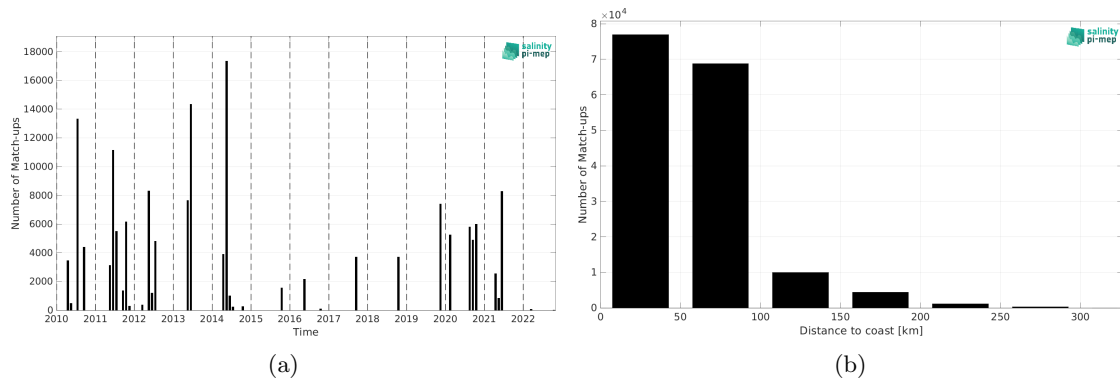
Figure 2: Number of match-ups between TSG (CSIC-UTM) and SMOS SSS L3 v335 - Monthly - 25 km (CATDS-CPDC) SSS as a function of time (a) and as function of the distance to coast (b) over the Mediterranean Sea Pi-MEP region and for the full satellite product period.
