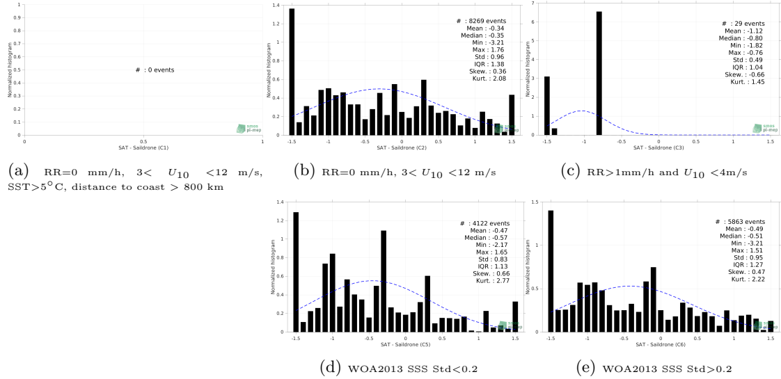
Figure 13: Normalized histogram of \Delta\text{SSS} (SMOS SSS L3 v335 - Monthly - 25 km (CATDS-CPDC) - Sailability) for 5 different subdatasets corresponding to: RR=0 mm/h, 3 < U_{10} < 12 m/s, SST > 5^\circ\text{C} , distance to coast > 800 km (a), RR=0 mm/h, 3 < U_{10} < 12 m/s (b), RR > 1\text{mm/h} and U_{10} < 4\text{m/s} (c), WOA2013 SSS Std < 0.2 (d), WOA2013 SSS Std > 0.2 (e).
