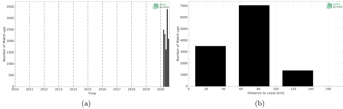
Figure 1: Number of match-ups between Saildrone and SMOS SSS L3 v335 - Monthly - 25 km (CATDS-CPDC) SSS as a function of time (a) and as function of the distance to coast (b) over the Mediterranean Sea Pi-MEP region and for the full satellite product period.
