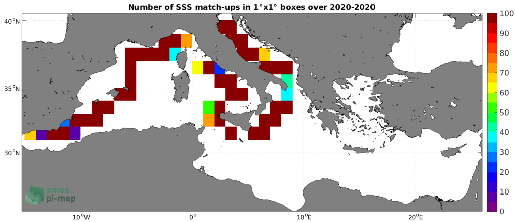
Figure 4: Number of SSS match-ups between Sairdrone SSS and the SMOS SSS L3 v335 - Monthly - 25 km (CATDS-CPDC) SSS product for the Mediterranean Sea Pi-MEP region over 1^\circ \times 1^\circ boxes and for the full satellite product period.
