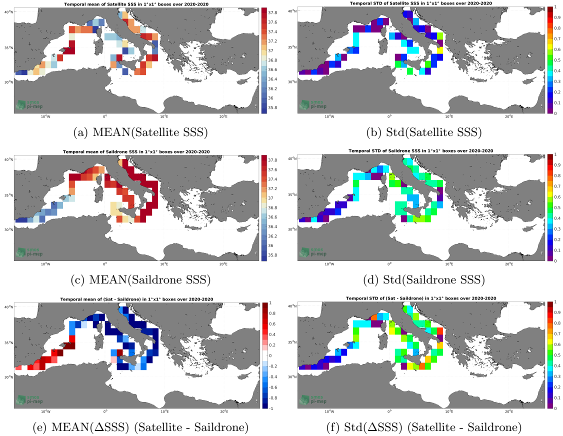
Figure 6: Temporal mean (left) and Std (right) of SSS from SMOS SSS L3 v335 - Monthly - 25 km (CATDS-CPDC) (top), Saildrone (middle), and of \Delta SSS (Satellite - Saildrone). Only match-up pairs are used to generate these maps.
