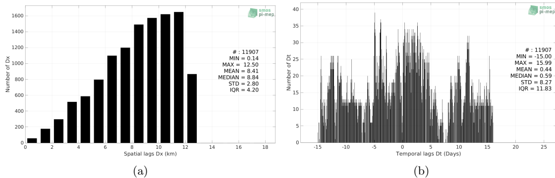
Figure 5: Histograms of the spatial (a) and temporal (b) lags between the location/time of the Sairdrone measurement and the date of the corresponding SMOS SSS L3 v335 - Monthly - 25 km (CATDS-CPDC) SSS pixel.
