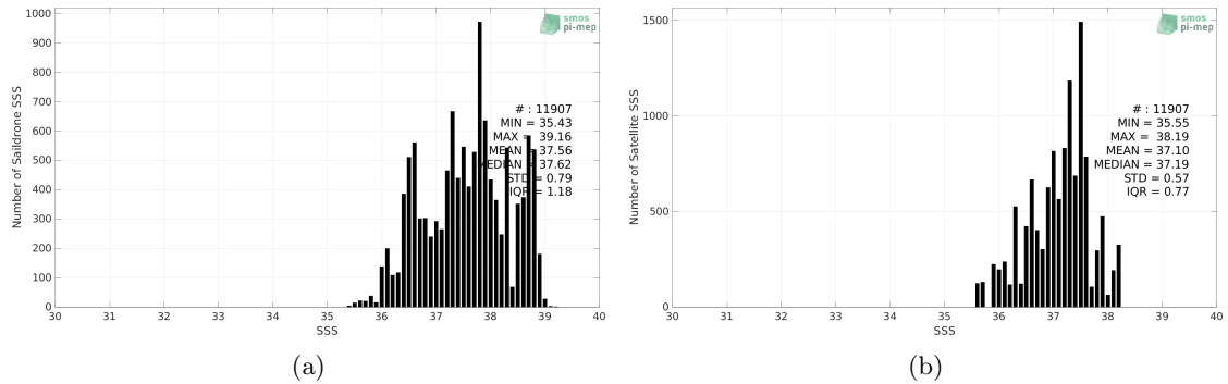
Figure 2: Histograms of SSS from Saildrone (a) and SMOS SSS L3 v335 - Monthly - 25 km (CATDS-CPDC) (b) considering all match-up pairs per bins of 0.1 over the Mediterranean Sea Pi-MEP region and for the full satellite product period.
