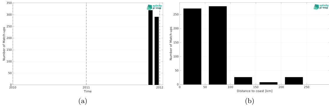
Figure 2: Number of match-ups between TSG (SAMOS) and SMOS SSS L3 v335 - 10 Days - 25 km (CATDS-CPDC) SSS as a function of time (a) and as function of the distance to coast (b) over the Mediterranean Sea Pi-MEP region and for the full satellite product period.
