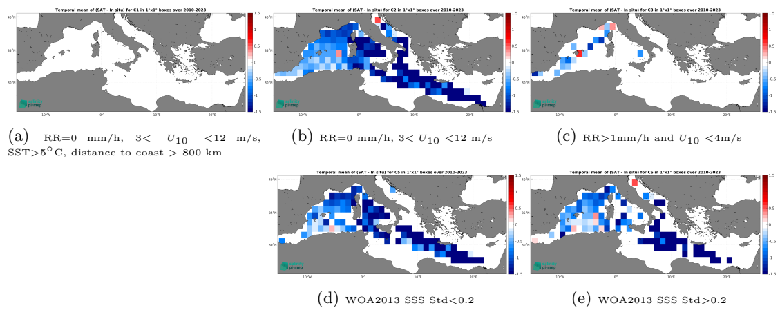
Figure 14: Temporal mean gridded over spatial boxes of size 1^\circ \times 1^\circ of \Delta SSS (SMOS SSS L3 v335 - 10 Days - 25 km (CATDS-CPDC) - TSG (LEGOS-DM)) for 5 different subdatasets corresponding to:RR=0 mm/h, 3 < U_{10} < 12 m/s, SST>5°C, distance to coast > 800 km (a), RR=0 mm/h, 3 < U_{10} < 12 m/s (b), RR>1mm/h and U_{10} < 4 m/s (c), WOA2013 SSS Std<0.2 (d), WOA2013 SSS Std>0.2 (e).
