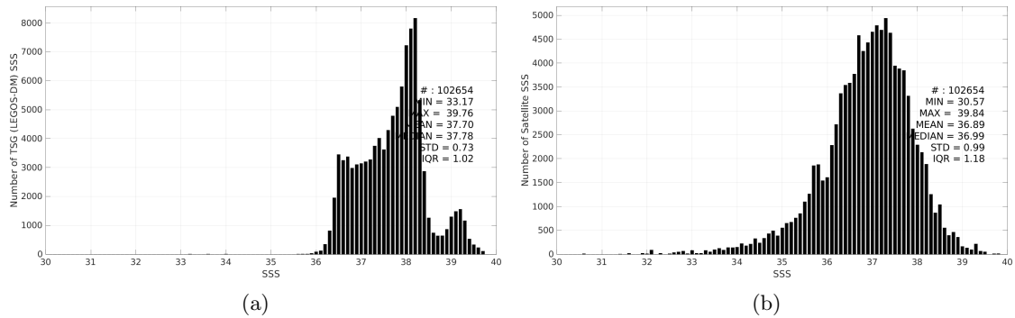
Figure 3: Histograms of SSS from TSG (LEGOS-DM) (a) and SMOS SSS L3 v335 - 10 Days - 25 km (CATDS-CPDC) (b) considering all match-up pairs per bins of 0.1 over the Mediterranean Sea Pi-MEP region and for the full satellite product period.
