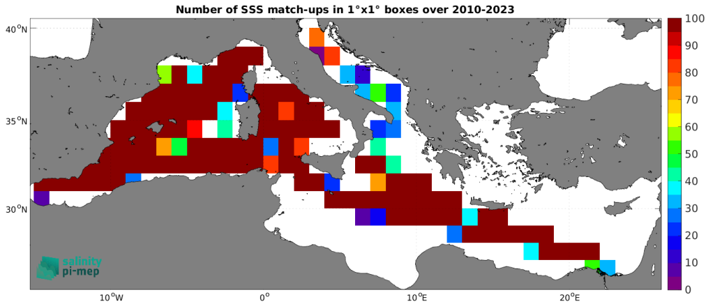
Figure 5: Number of SSS match-ups between TSG (LEGOS-DM) SSS and the SMOS SSS L3 v335 - 10 Days - 25 km (CATDS-CPDC) SSS product for the Mediterranean Sea Pi-MEP region over 1^\circ \times 1^\circ boxes and for the full satellite product period.
