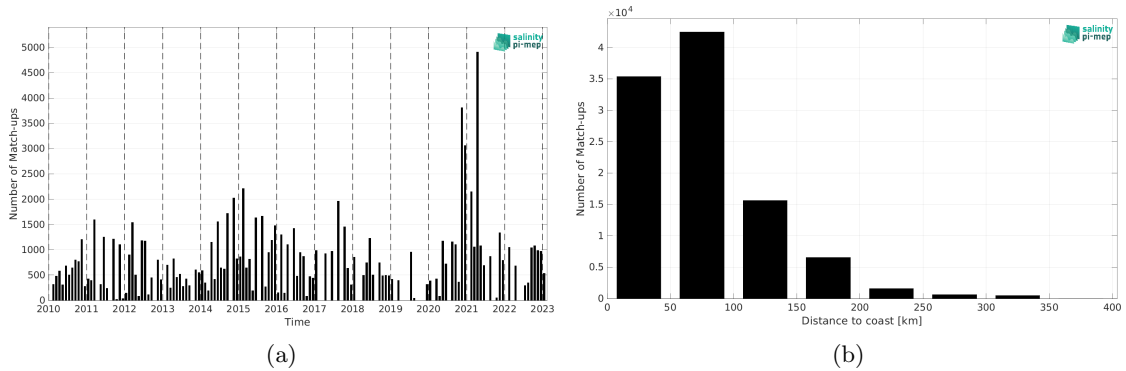
Figure 2: Number of match-ups between TSG (LEGOS-DM) and SMOS SSS L3 v335 - 10 Days - 25 km (CATDS-CPDC) SSS as a function of time (a) and as function of the distance to coast (b) over the Mediterranean Sea Pi-MEP region and for the full satellite product period.
