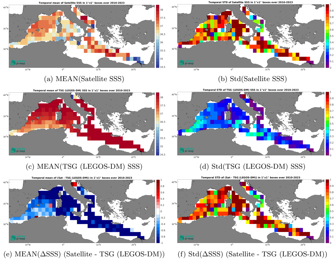
Figure 7: Temporal mean (left) and Std (right) of SSS from SMOS SSS L3 v335 - 10 Days - 25 km (CATDS-CPDC) (top), TSG (LEGOS-DM) (middle), and of \Delta\text{SSS} (Satellite - TSG (LEGOS-DM)). Only match-up pairs are used to generate these maps.
