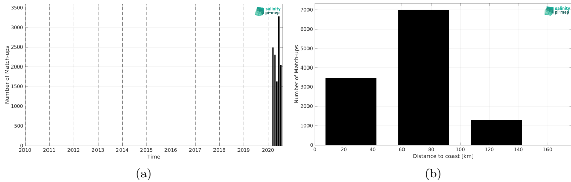
Figure 2: Number of match-ups between Saildrone and SMOS SSS L3 v335 - 10 Days - 25 km (CATDS-CPDC) SSS as a function of time (a) and as function of the distance to coast (b) over the Mediterranean Sea Pi-MEP region and for the full satellite product period.
