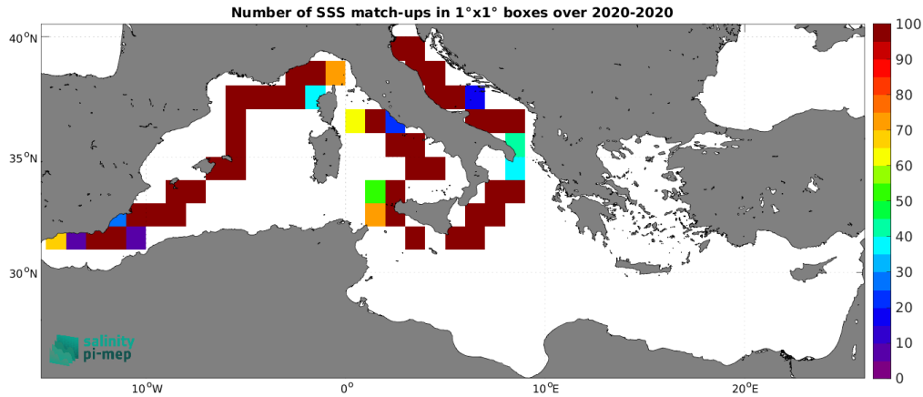
Figure 5: Number of SSS match-ups between Saildrone SSS and the SMOS SSS L3 v335 - 10 Days - 25 km (CATDS-CPDC) SSS product for the Mediterranean Sea Pi-MEP region over 1^\circ \times 1^\circ boxes and for the full satellite product period.
