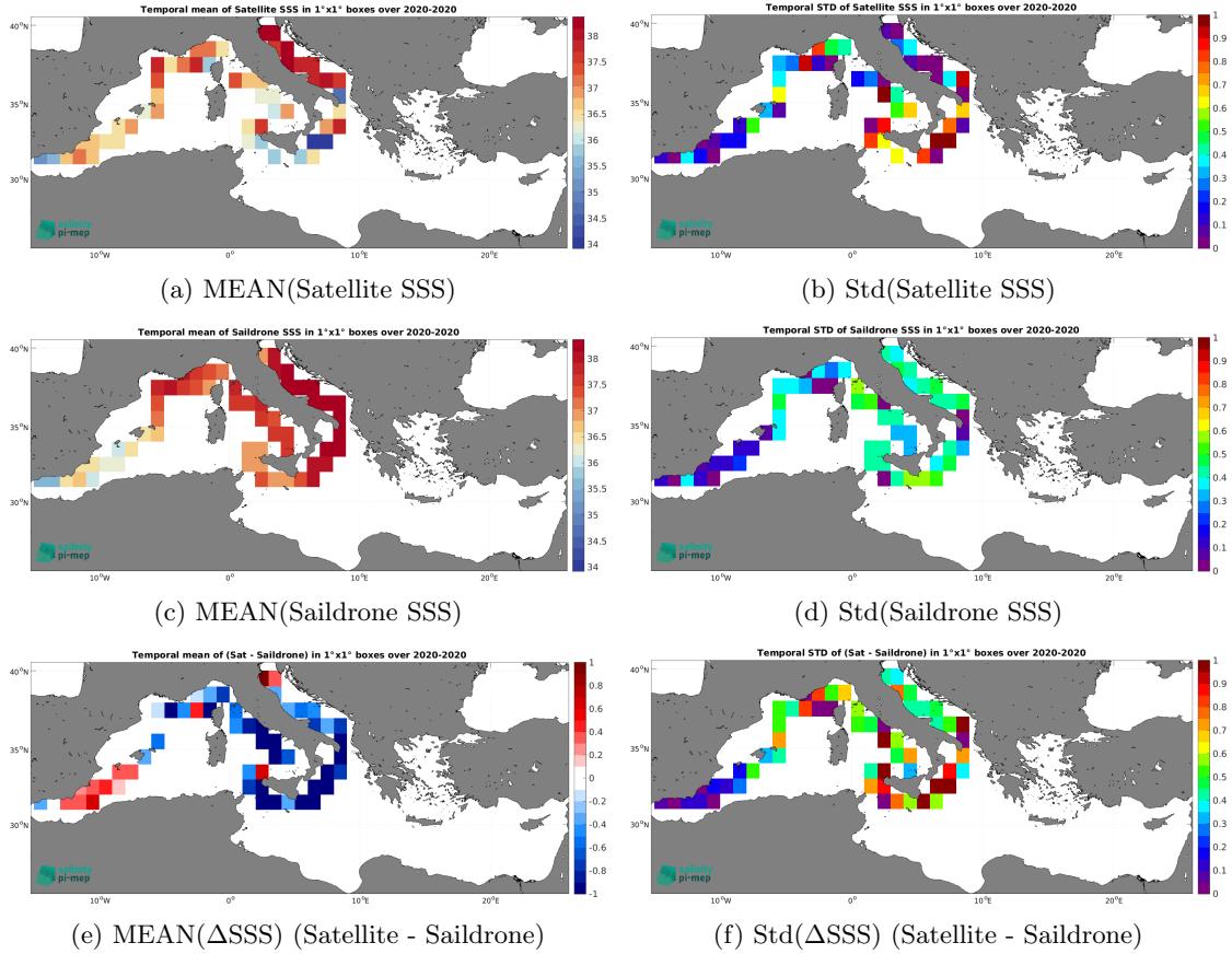
Figure 7: Temporal mean (left) and Std (right) of SSS from SMOS SSS L3 v335 - 10 Days - 25 km (CATDS-CPDC) (top), Saildrone (middle), and of \Delta SSS (Satellite - Saildrone). Only match-up pairs are used to generate these maps.
