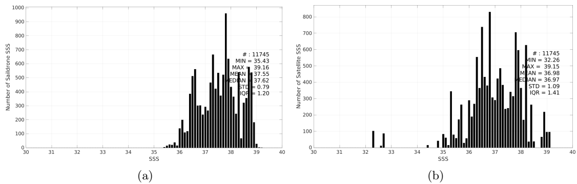
Figure 3: Histograms of SSS from Saildrone (a) and SMOS SSS L3 v335 - 10 Days - 25 km (CATDS-CPDC) (b) considering all match-up pairs per bins of 0.1 over the Mediterranean Sea Pi-MEP region and for the full satellite product period.
