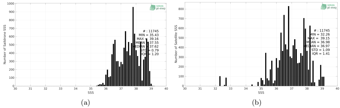
Figure 2: Histograms of SSS from Saildrone (a) and SMOS SSS L3 v335 - 10 Days - 25 km (CATDS-CPDC) (b) considering all match-up pairs per bins of 0.1 over the Mediterranean Sea Pi-MEP region and for the full satellite product period.
