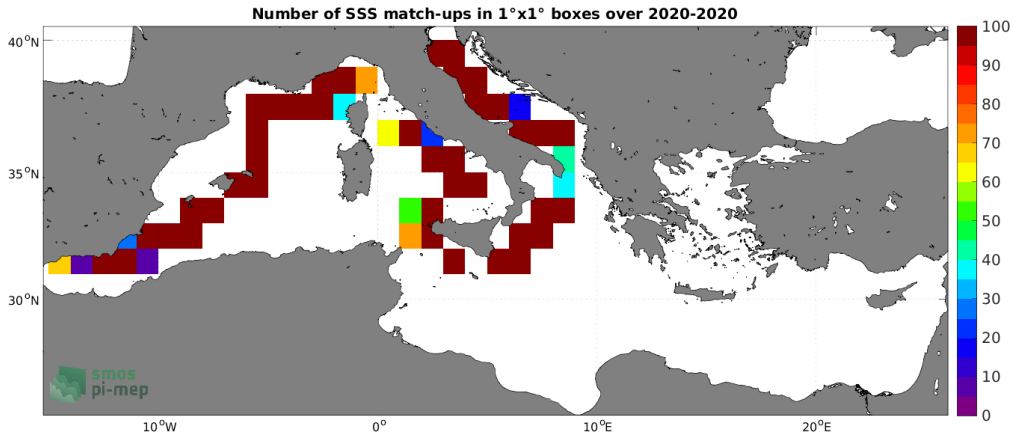
Figure 4: Number of SSS match-ups between Saildrone SSS and the SMOS SSS L3 v335 - 10 Days - 25 km (CATDS-CPDC) SSS product for the Mediterranean Sea Pi-MEP region over 1^\circ \times 1^\circ boxes and for the full satellite product period.
