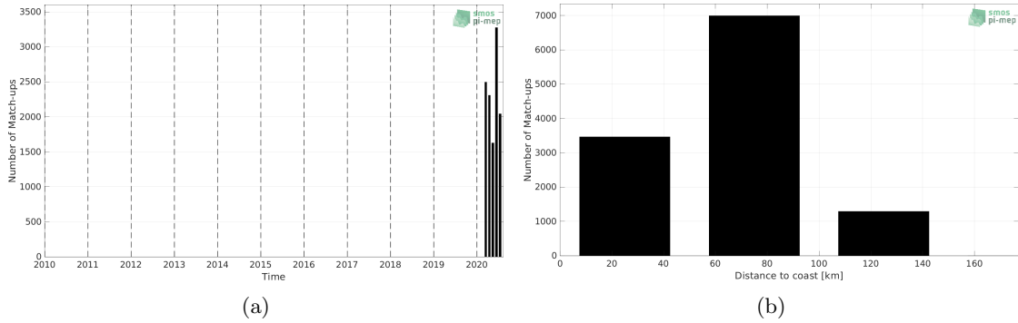
Figure 1: Number of match-ups between Saildrone and SMOS SSS L3 v335 - 10 Days - 25 km (CATDS-CPDC) SSS as a function of time (a) and as function of the distance to coast (b) over the Mediterranean Sea Pi-MEP region and for the full satellite product period.
