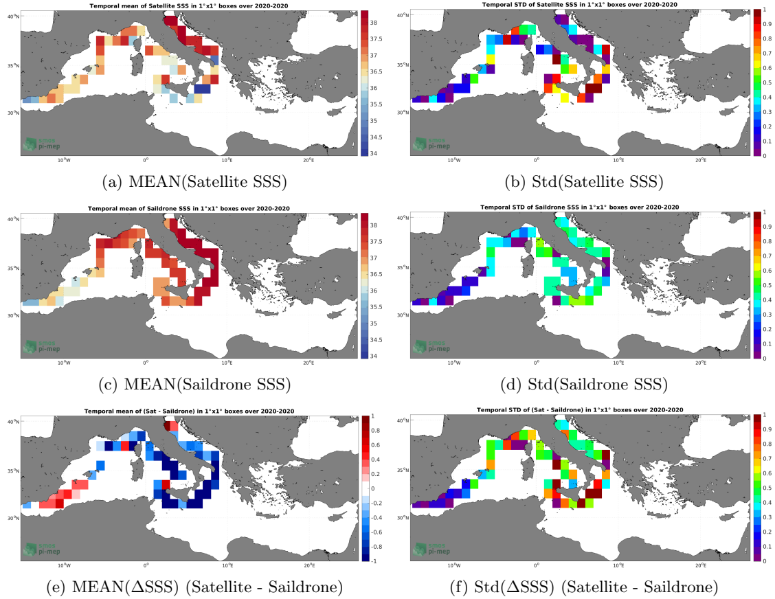
Figure 6: Temporal mean (left) and Std (right) of SSS from SMOS SSS L3 v335 - 10 Days - 25 km (CATDS-CPDC) (top), Saildrone (middle), and of \Delta SSS (Satellite - Saildrone). Only match-up pairs are used to generate these maps.
