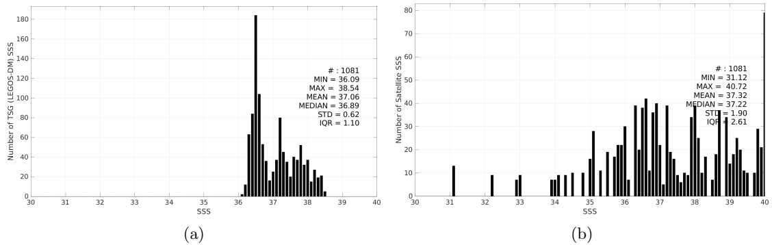
Figure 3: Histograms of SSS from TSG (LEGOS-DM) (a) and SMOS SSS L2Q v333 - 0.25 Deg (CATDS-CPDC) (b) considering all match-up pairs per bins of 0.1 over the Mediterranean Sea Pi-MEP region and for the full satellite product period.
