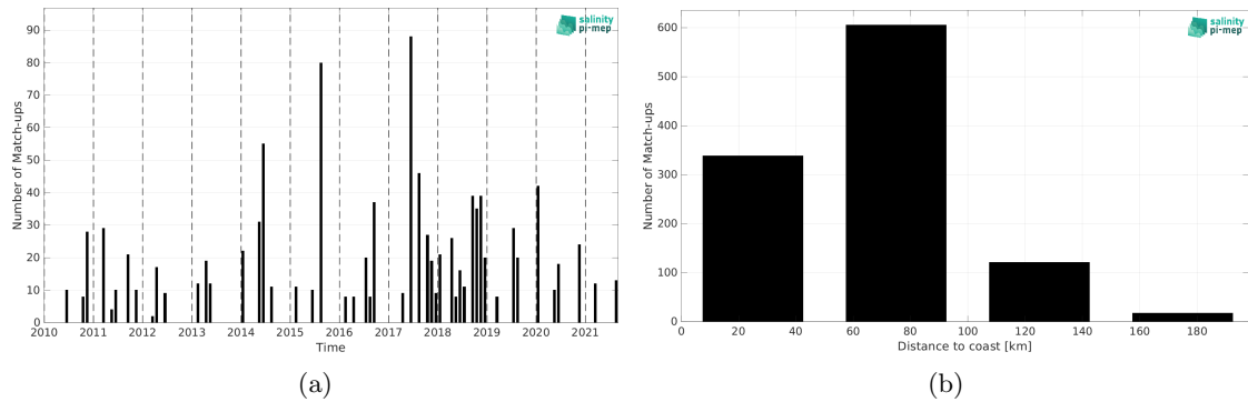
Figure 2: Number of match-ups between TSG (LEGOS-DM) and SMOS SSS L2Q v333 - 0.25 Deg (CATDS-CPDC) SSS as a function of time (a) and as function of the distance to coast (b) over the Mediterranean Sea Pi-MEP region and for the full satellite product period.
