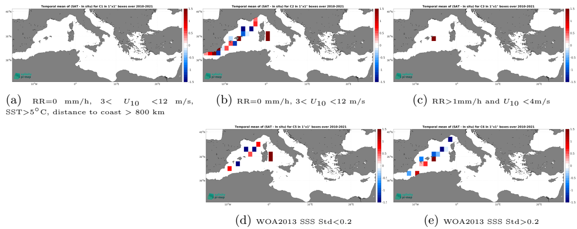
Figure 14: Temporal mean gridded over spatial boxes of size 1^\circ \times 1^\circ of \Delta SSS (SMOS SSS L2Q v333 - 0.25 Deg (CATDS-CPDC) - TSG (LEGOS-DM)) for 5 different subdatasets corresponding to:RR=0 mm/h, 3 < U_{10} < 12 m/s, SST>5°C, distance to coast > 800 km (a), RR=0 mm/h, 3 < U_{10} < 12 m/s (b), RR>1mm/h and U_{10} < 4 m/s (c), WOA2013 SSS Std<0.2 (d), WOA2013 SSS Std>0.2 (e).
