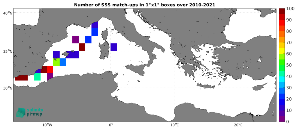
Figure 5: Number of SSS match-ups between TSG (LEGOS-DM) SSS and the SMOS SSS L2Q v333 - 0.25 Deg (CATDS-CPDC) SSS product for the Mediterranean Sea Pi-MEP region over 1^\circ \times 1^\circ boxes and for the full satellite product period.
