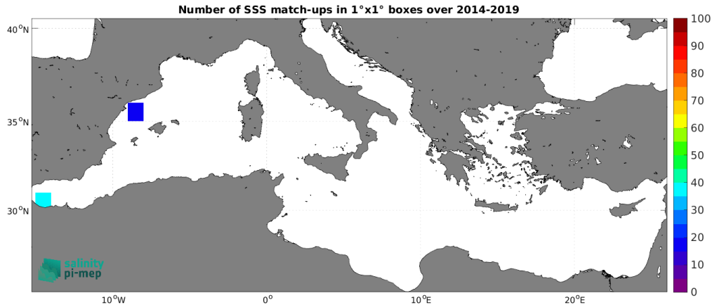
Figure 5: Number of SSS match-ups between TSG (GOSUD-Sailing-ship) SSS and the SMOS SSS L2Q v333 - 0.25 Deg (CATDS-CPDC) SSS product for the Mediterranean Sea Pi-MEP region over 1^\circ \times 1^\circ boxes and for the full satellite product period.
