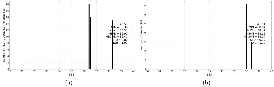
Figure 3: Histograms of SSS from TSG (GOSUD-Sailing-ship) (a) and SMOS SSS L2Q v333 - 0.25 Deg (CATDS-CPDC) (b) considering all match-up pairs per bins of 0.1 over the Mediterranean Sea Pi-MEP region and for the full satellite product period.
