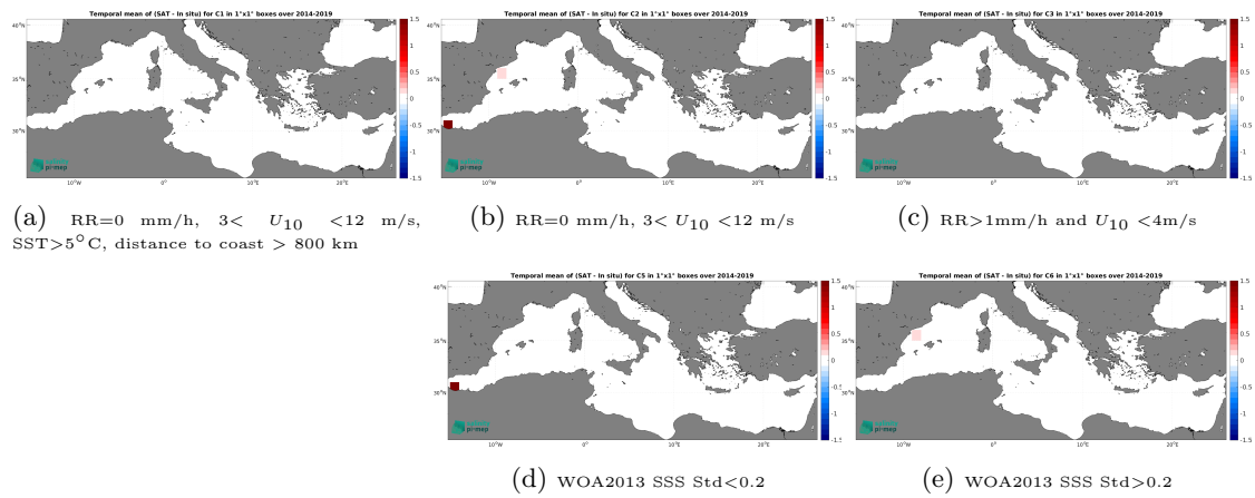
Figure 14: Temporal mean gridded over spatial boxes of size 1^\circ \times 1^\circ of \Delta SSS (SMOS SSS L2Q v333 - 0.25 Deg (CATDS-CPDC) - TSG (GOSUD-Sailing-ship)) for 5 different subdatasets corresponding to: RR=0 mm/h, 3 < U_{10} < 12 m/s, SST > 5°C, distance to coast > 800 km (a), RR=0 mm/h, 3 < U_{10} < 12 m/s (b), RR > 1 mm/h and U_{10} < 4 m/s (c), WOA2013 SSS Std < 0.2 (d), WOA2013 SSS Std > 0.2 (e).
