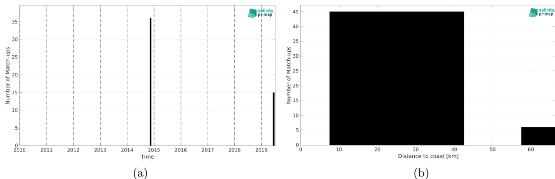
Figure 2: Number of match-ups between TSG (GOSUD-Sailing-ship) and SMOS SSS L2Q v333 - 0.25 Deg (CATDS-CPDC) SSS as a function of time (a) and as function of the distance to coast (b) over the Mediterranean Sea Pi-MEP region and for the full satellite product period.
