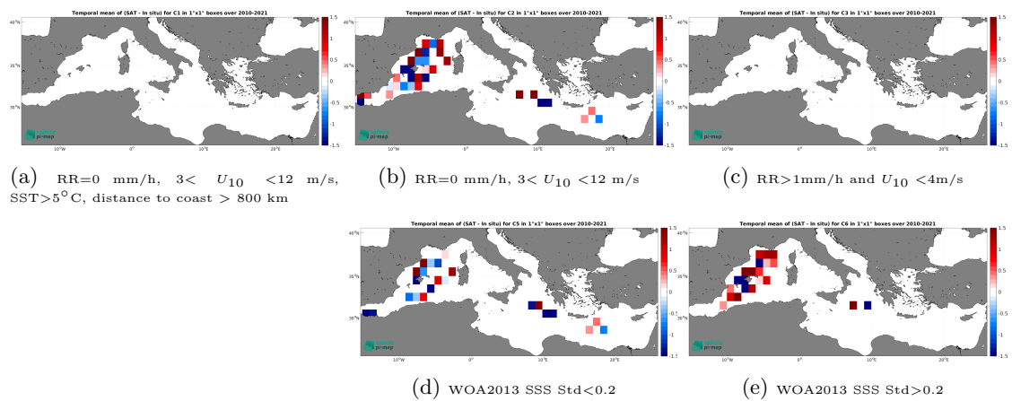
Figure 14: Temporal mean gridded over spatial boxes of size 1^\circ \times 1^\circ of \Delta SSS (SMOS SSS L2Q v333 - 0.25 Deg (CATDS-CPDC) - TSG (GOSUD-Research-vessel)) for 5 different subdatasets corresponding to:RR=0 mm/h, 3 < U_{10} < 12 m/s, SST>5°C, distance to coast > 800 km (a), RR=0 mm/h, 3 < U_{10} < 12 m/s (b), RR>1mm/h and U_{10} < 4 m/s (c), WOA2013 SSS Std<0.2 (d), WOA2013 SSS Std>0.2 (e).
