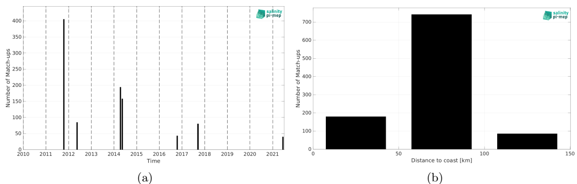
Figure 2: Number of match-ups between TSG (CSIC-UTM) and SMOS SSS L2Q v333 - 0.25 Deg (CATDS-CPDC) SSS as a function of time (a) and as function of the distance to coast (b) over the Mediterranean Sea Pi-MEP region and for the full satellite product period.
