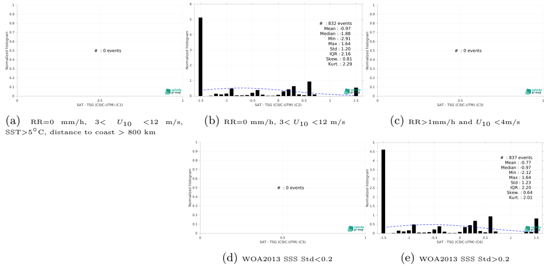
Figure 15: Normalized histogram of \Delta\text{SSS} (SMOS SSS L2Q v333 - 0.25 Deg (CATDS-CPDC) - TSG (CSIC-UTM)) for 5 different subdatasets corresponding to: RR=0 mm/h, 3 < U_{10} < 12 m/s, SST > 5^{\circ}\text{C} , distance to coast > 800 km (a), RR=0 mm/h, 3 < U_{10} < 12 m/s (b), RR > 1\text{mm/h} and U_{10} < 4\text{m/s} (c), WOA2013 SSS Std < 0.2 (d), WOA2013 SSS Std > 0.2 (e).
