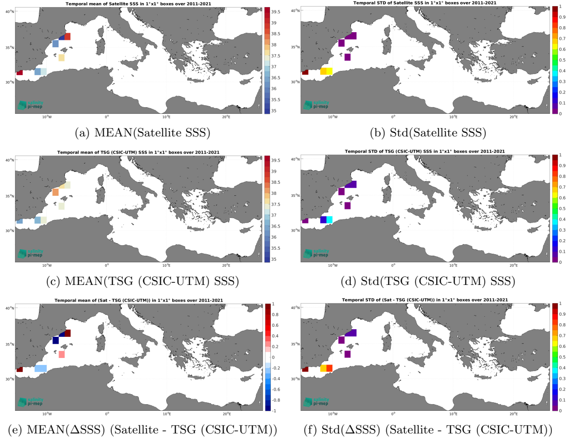
Figure 7: Temporal mean (left) and Std (right) of SSS from SMOS SSS L2Q v333 - 0.25 Deg (CATDS-CPDC) (top), TSG (CSIC-UTM) (middle), and of \Delta\text{SSS} (Satellite - TSG (CSIC-UTM)). Only match-up pairs are used to generate these maps.
