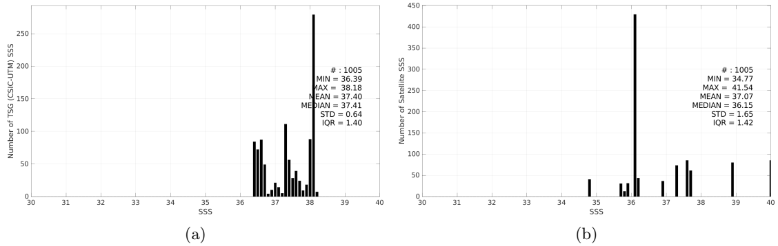
Figure 3: Histograms of SSS from TSG (CSIC-UTM) (a) and SMOS SSS L2Q v333 - 0.25 Deg (CATDS-CPDC) (b) considering all match-up pairs per bins of 0.1 over the Mediterranean Sea Pi-MEP region and for the full satellite product period.
