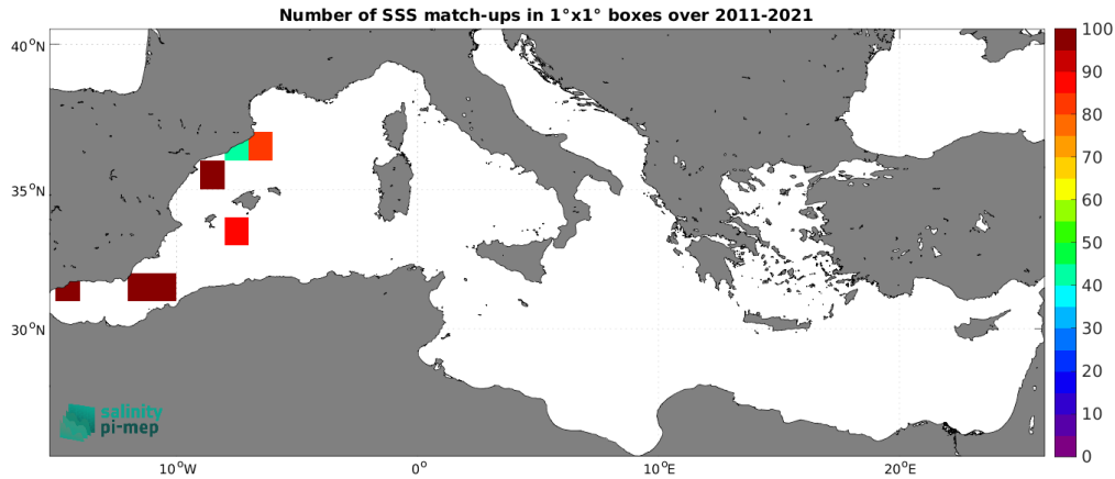
Figure 5: Number of SSS match-ups between TSG (CSIC-UTM) SSS and the SMOS SSS L2Q v333 - 0.25 Deg (CATDS-CPDC) SSS product for the Mediterranean Sea Pi-MEP region over 1^\circ \times 1^\circ boxes and for the full satellite product period.
