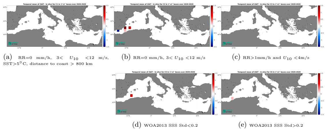
Figure 14: Temporal mean gridded over spatial boxes of size 1^\circ \times 1^\circ of \Delta SSS (SMOS SSS L2Q v333 - 0.25 Deg (CATDS-CPDC) - Saildrone) for 5 different subdatasets corresponding to:RR=0 mm/h, 3 < U_{10} < 12 m/s, SST >5^\circ\text{C} , distance to coast > 800 km (a), RR=0 mm/h, 3 < U_{10} < 12 m/s (b), RR >1 mm/h and U_{10} < 4 m/s (c), WOA2013 SSS Std <0.2 (d), WOA2013 SSS Std >0.2 (e).
