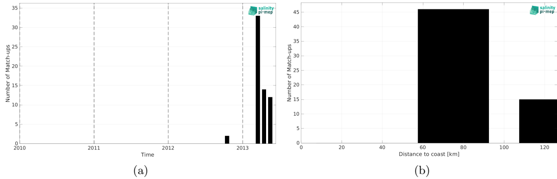
Figure 2: Number of match-ups between Surface drifters and SMOS SSS L2Q v333 - 0.25 Deg (CATDS-CPDC) SSS as a function of time (a) and as function of the distance to coast (b) over the Mediterranean Sea Pi-MEP region and for the full satellite product period.
