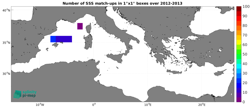
Figure 4: Number of SSS match-ups between Surface drifters SSS and the SMOS SSS L2Q v333 - 0.25 Deg (CATDS-CPDC) SSS product for the Mediterranean Sea Pi-MEP region over 1^\circ \times 1^\circ boxes and for the full satellite product period.
