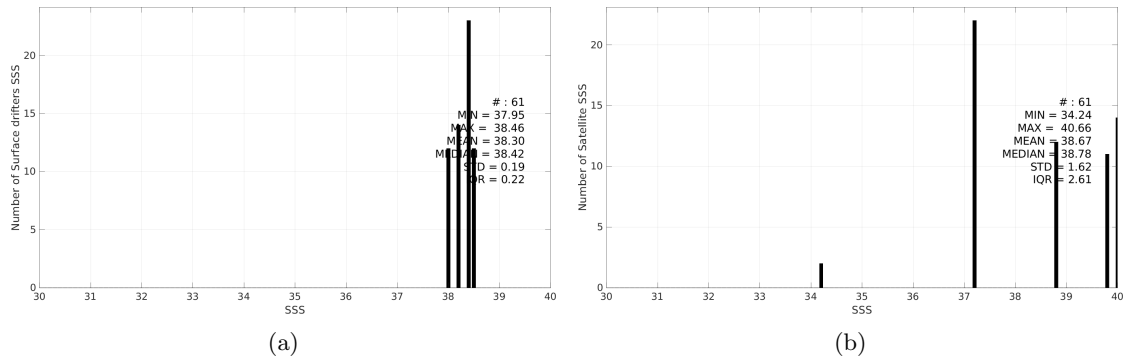
Figure 3: Histograms of SSS from Surface drifters (a) and SMOS SSS L2Q v333 - 0.25 Deg (CATDS-CPDC) (b) considering all match-up pairs per bins of 0.1 over the Mediterranean Sea Pi-MEP region and for the full satellite product period.
